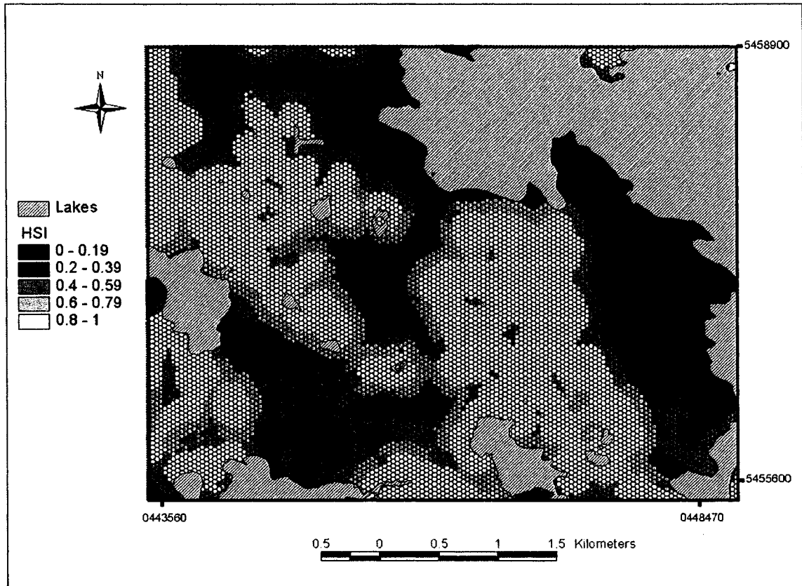
Figure 1.2. Example of a Habitat Suitability Index (HSI) model of part of the Cameron Lake area in northwestern Ontario showing resource suitability for elk within hexagons. Lighter shaded hexagons indicate better quality resources than darker shades.
