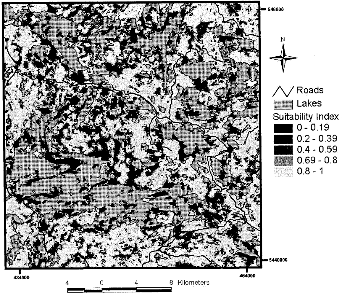
Figure 3.5. Resource suitability map based on the RUF model for the Cameron Lake area. Darker shades represent lower elk resource suitability.
