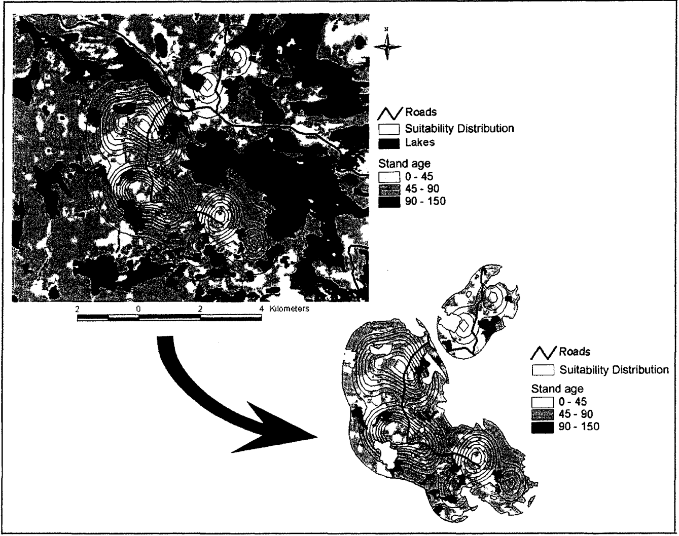
Figure 2.2. Example of a clipped suitability distribution with calculated landscape metrics and without lakes.
