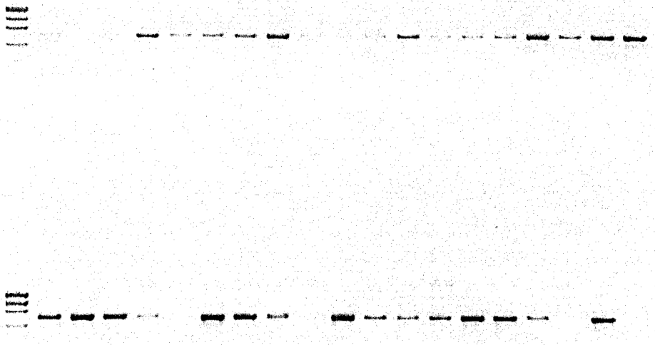
Figure 1.1. Amplification of mtDNA control region using agarose gel stained with ethidium bromide for a subset of caribou faecal samples collected in the summer of 2004.
