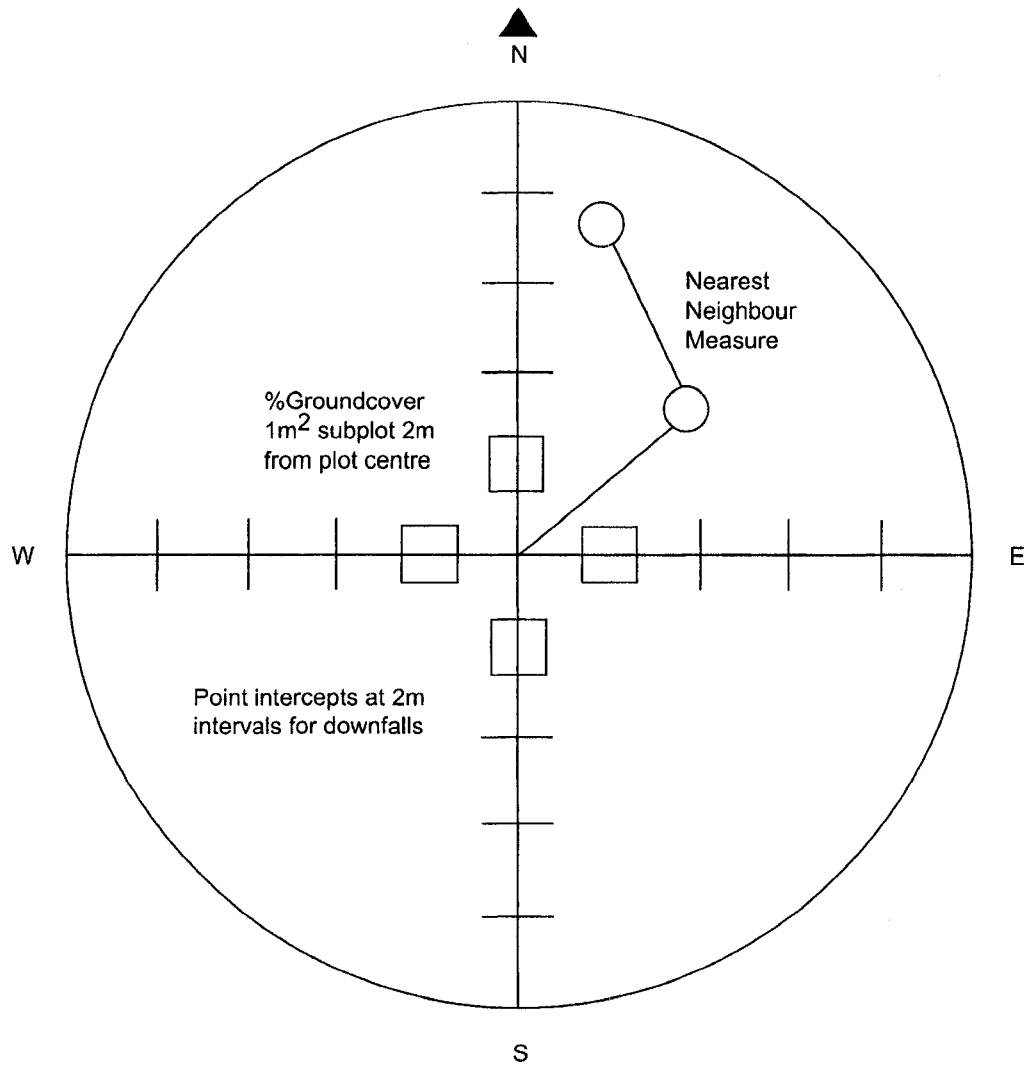
Figure 2.2. Schematic of detailed vegetation measurements made within 10m-radius sampling plots at caribou nursery sites and randomly chosen absence sites on lakes in Wabakimi and Woodland Caribou Provincial Parks, northern Ontario.
