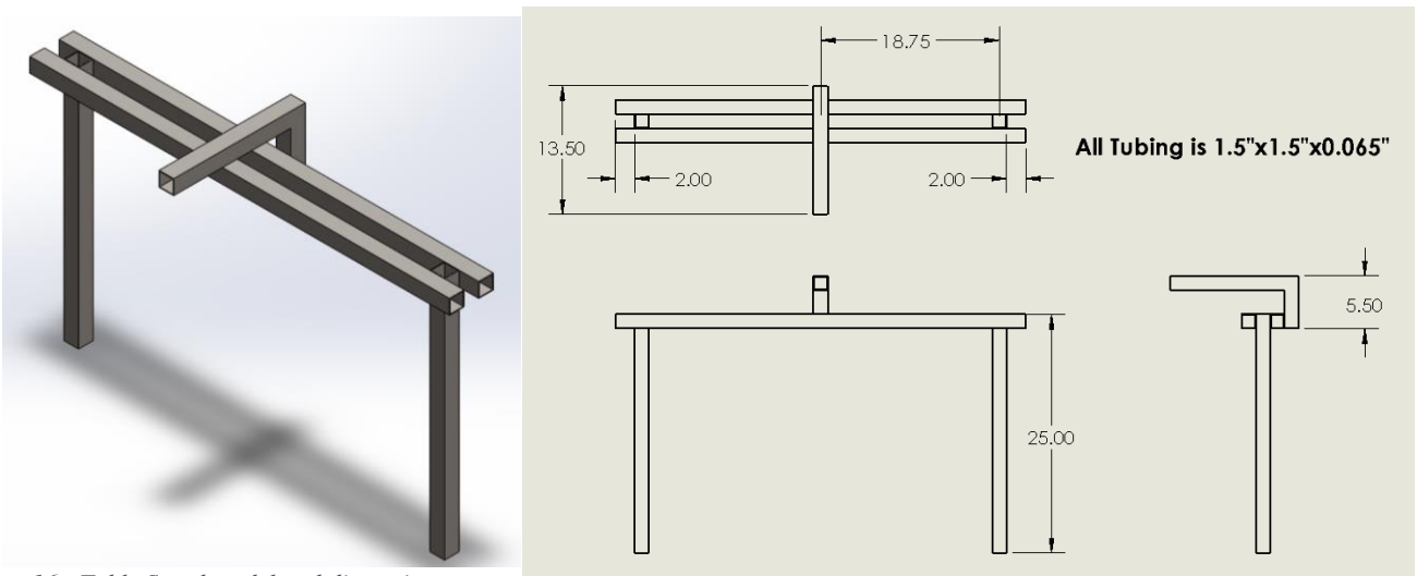
Figure 16 - Table Stand model and dimensions
