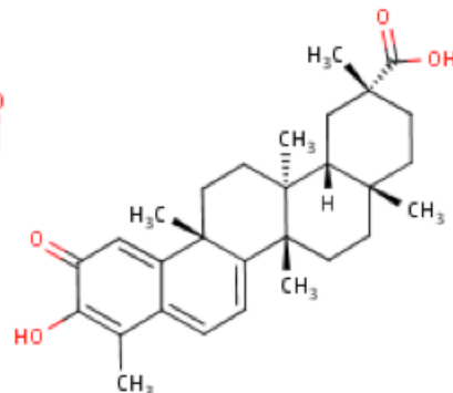
Figure 3. Celestrol ( C_{29}H_{38}O_4 , MW: 450.6152)
