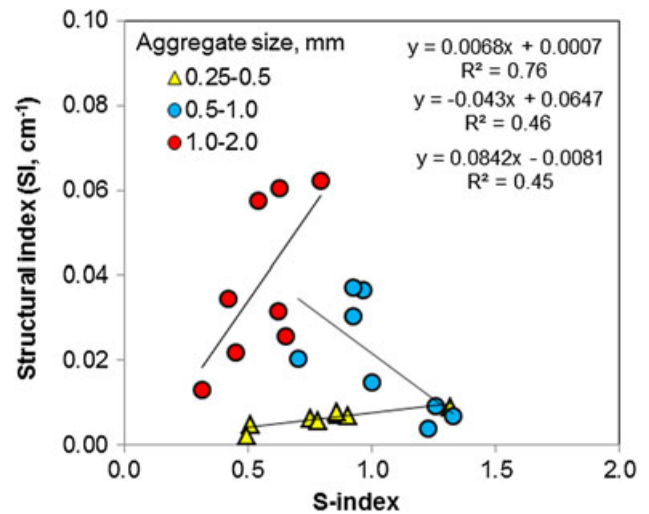
Figure 10. Structural index (SI) as a function of S-index, the slope of the water retention curve in its inflection point. [Colour figure can be viewed at wileyonlinelibrary.com ]
