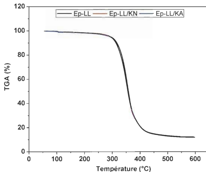
Figure III.58 Courbes TGA des composites hybrides lin/Kraft/époxy.
