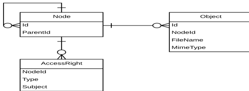
Figure 2: Node and objects relations
