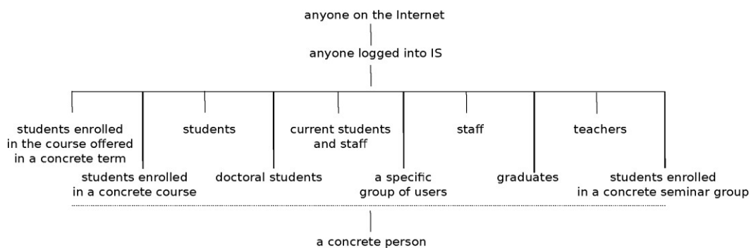
Figure 1: Hierarchy of access rights
