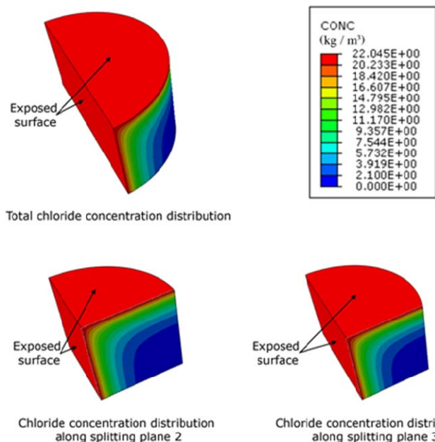
Fig. 11. Chloride concentration distribution [14]
