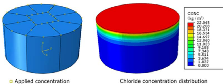
Fig. 8. Applied boundary conditions and chloride concentration distribution [14]
