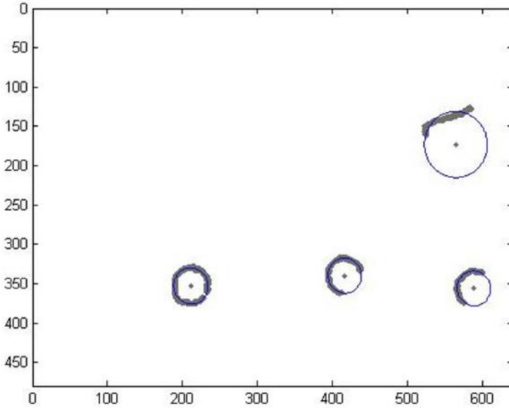
Fig. 10 Circle approximation via segments
