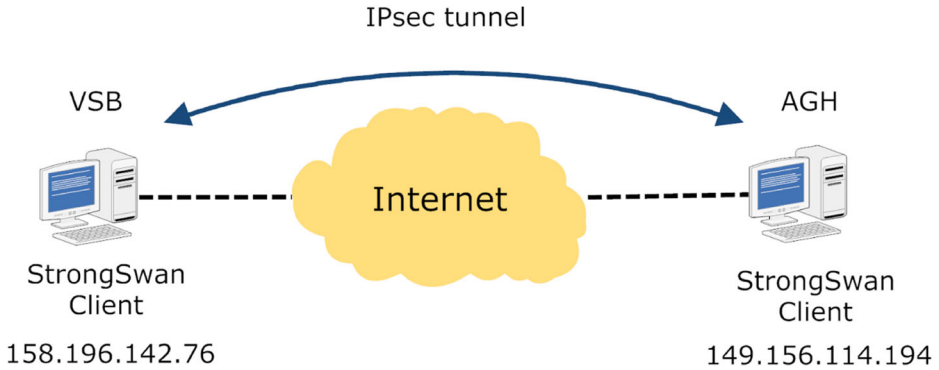
Fig. 1 Test topology
