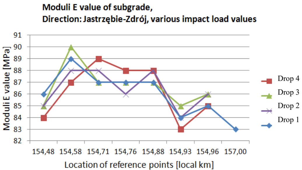
Fig.9: Value of backcalculated moduli subgrade on left lane (Jastrzębie-Zdrój direction)
