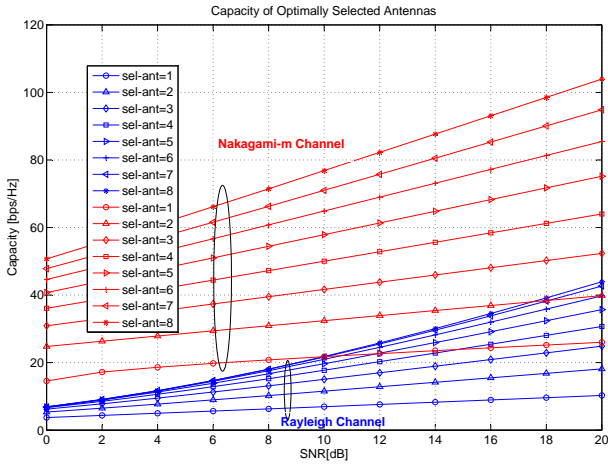
Fig. 3: Channel capacity with optimal antenna selection: N_T = N_R = 8 and \text{sel} - \text{ant} = 1, 2, 3, 4, 5, 6, 7, 8 .
