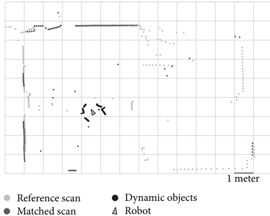
FIGURE 8: Dynamic objects robustness.
