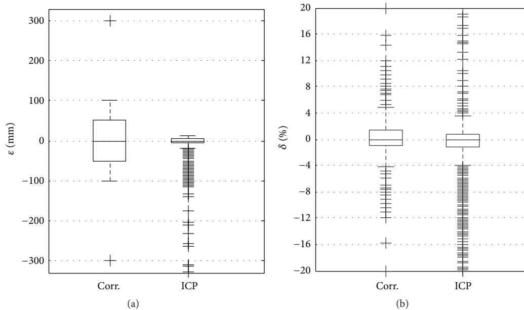
FIGURE 10: Error comparison: (a) absolute error, (b) relative error.
