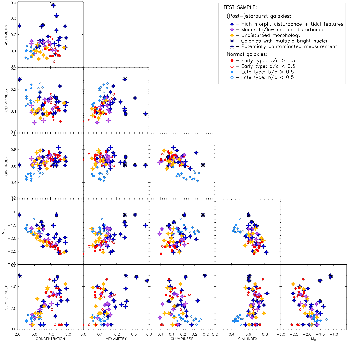
Figure 4. Relations between the six standard morphology measures (Sérsic index [ n ], concentration [ C ], asymmetry [ A ], clumpiness [ S ], Gini index [ G ] and M_{20} ) computed for the test sample. The meaning of the symbols is described in the legend where galaxies are split into subsets based on visual classification and the SDSS fracdev parameter (see Section 2.1).
