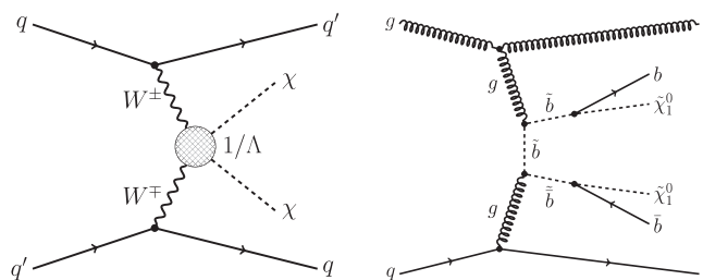
FIG. 1. Feynman diagrams for dark matter pair production in a vector boson fusion process (left) and for bottom squark pair production (right). Given a nearly degenerate bottom squark and LSP, the final-state b quarks are too soft to be observed.
