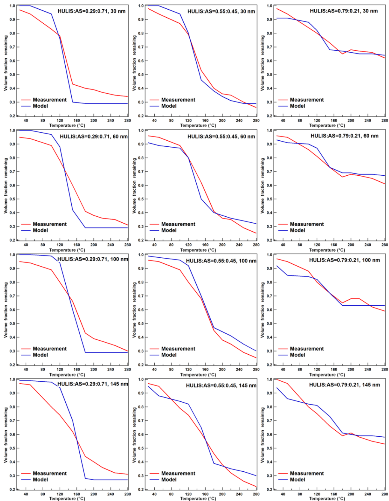
Figure 7. Measured and modeled volume fraction remaining (VFR) as a function of temperature for HULIS-AS mixed samples of three different mixing ratios at four different particle sizes of 30, 60, 100 and 145 nm.
