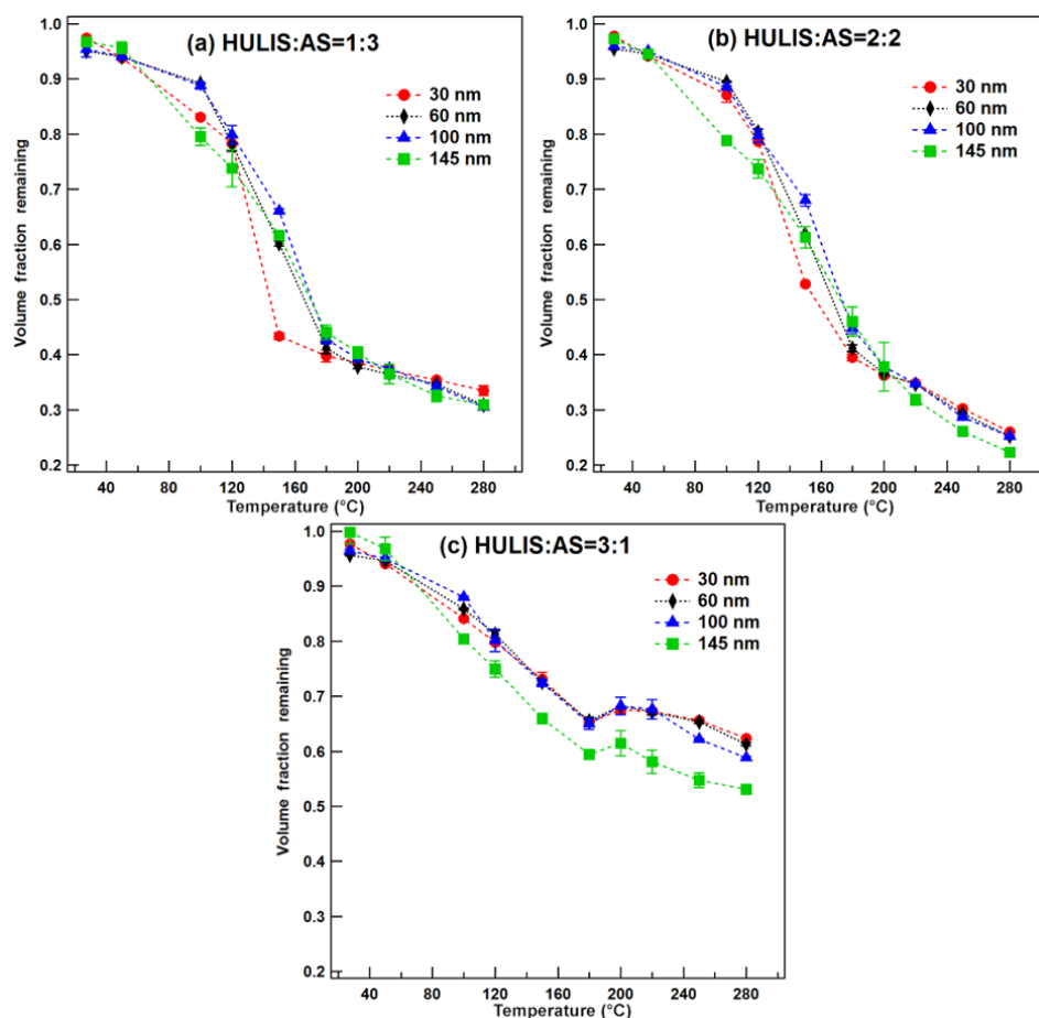
Figure 6. Volume fraction remaining (VFR) as a function of heating temperature for (a) 1 : 3 HULIS-AS mixed sample, (b) 2 : 2 HULIS-AS mixed samples, and (c) 3 : 1 HULIS-AS mixed samples at four different sizes of 30, 60, 100, and 145 nm.
