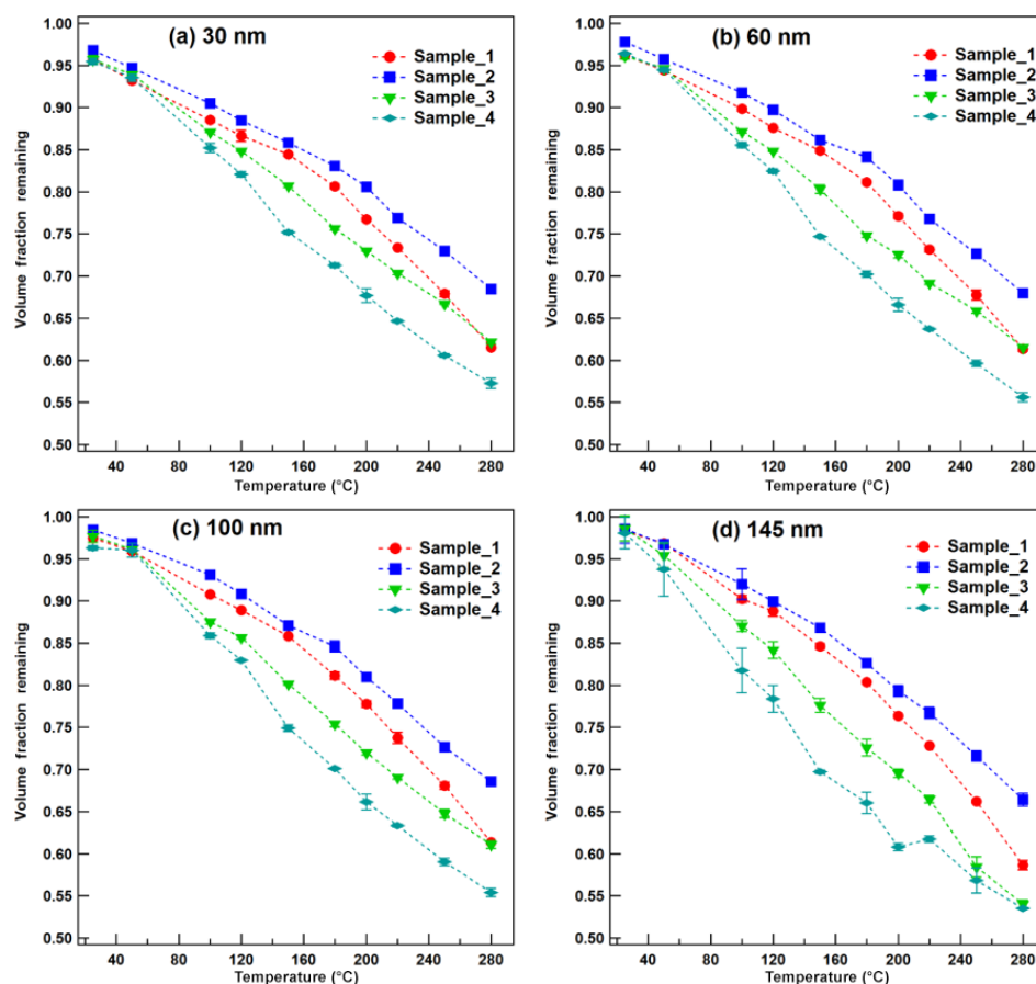
Figure 2. Volume fraction remaining (VFR) as a function of heating temperature for four samples at four different sizes of (a) 30 nm, (b) 60 nm, (c) 100 nm, and (d) 145 nm.
