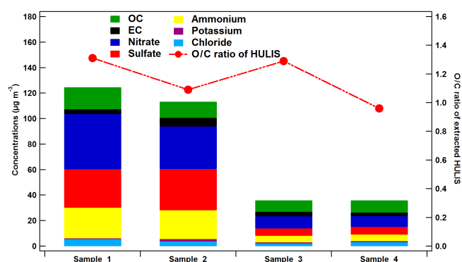
Figure 1. Chemical composition of the four \text{PM}_{2.5} samples collected at SORPES station and oxygen to carbon ratio of extracted HULIS from related samples.
