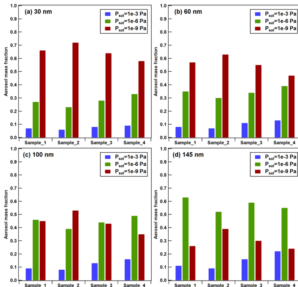
Figure 4. Mass fractions of compounds of SVOC ( p_{\text{sat}} = 10^{-3} Pa), LVOC ( p_{\text{sat}} = 10^{-6} Pa) and ELVOC ( p_{\text{sat}} = 10^{-9} Pa) in four aerosol samples with different particle sizes of (a) 30 nm, (b) 60 nm, (c) 100 nm, and (d) 145 nm.
