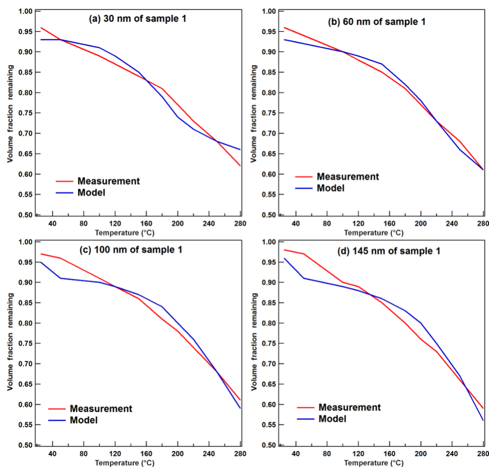
Figure 3. Measured and modeled volume fraction remaining (VFR) as a function of temperature for HULIS of sample 1 at four different particle sizes of (a) 30 nm, (b) 60 nm, (c) 100 nm, and (d) 145 nm.
