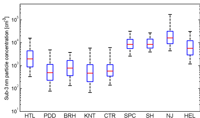
Figure 2. The variation in sub-3 nm particle concentration at different measurement sites. The red lines show the medians, the blue boxes indicate the 25th and 75th percentiles, and the vertical bars show the 5th and 95th percentiles.
