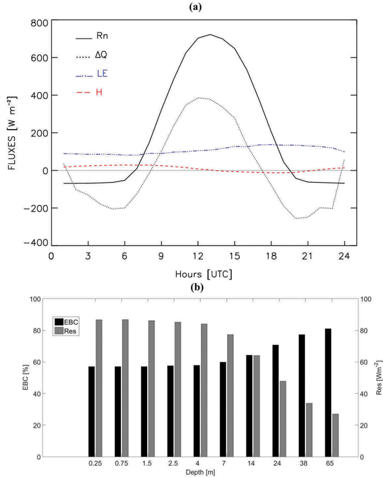
Fig. 7. (a) Mean daily cycle of net radiation ( R_n ), water column heat storage ( \Delta Q ), latent heat flux ( LE ) and sensible heat flux ( H ) during the period June–September 2014. (b) Average energy residual ( Res ) measured with different depths for water column heat storage ( \Delta Q ) calculations during the period June–September 2014. EBC = energy balance closure.
