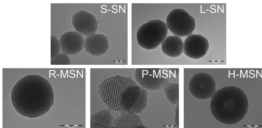
Fig. 1 TEM pictures and descriptions of different silica nanoparticles used in the study
