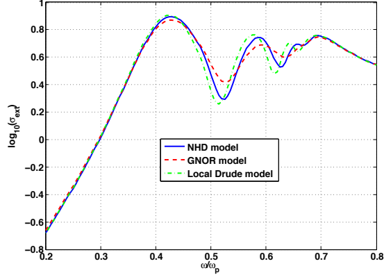
Figure 7: Comparison of extinction cross sections of a gold dimer as calculated with the local Drude model, the NHD model and the GNOR model. The configuration is shown in Figure 6 and the material parameters are given in subsection 4.3.
