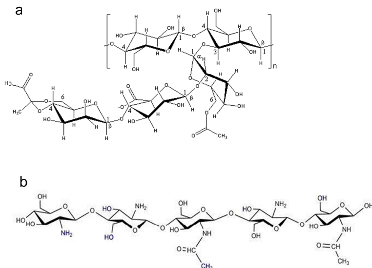
Figure 1. Chemical structure of (a) xanthan repeating unit and b) a representative structure of a chitosan pentamer, showing residues of \beta(1,4) -linked 2-amino-2-deoxy-D-glucose (D residues) and N-acetyl-2-amino-2-deoxy-D-glucose (A residues) (for clarity, single H in the sugar ring structure are not shown).
