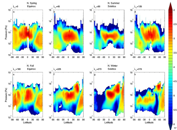
Figure 2. Log 10 of the day-side retrievals of zonal average water ice density-scaled opacity (m 2 kg -1 ), for MY29. the L S bins are labelled at the top of each panel, and the contours are shown every 0.1 log units (McCleese et al. , 2010).
