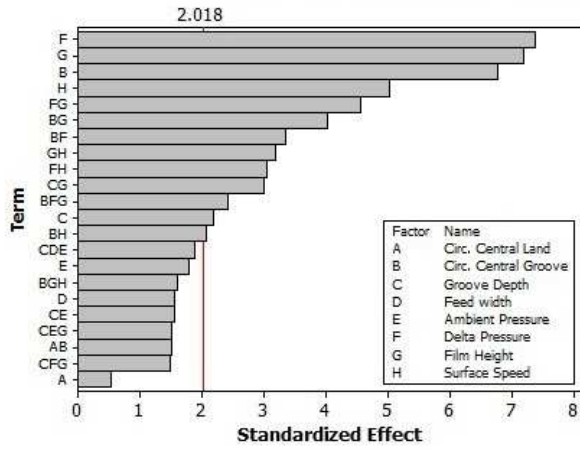
Fig. 10. Reduced model Pareto chart dimensionless stiffness
