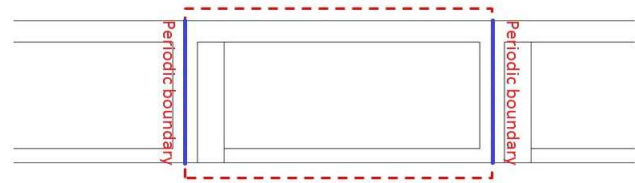
Fig. 5. Modelled section and repeating groove pattern
