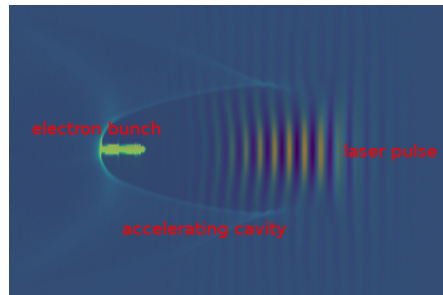
Figure 2. Electron bunch trapped in plasma cavity created behind the laser pulse during wakefield acceleration.
