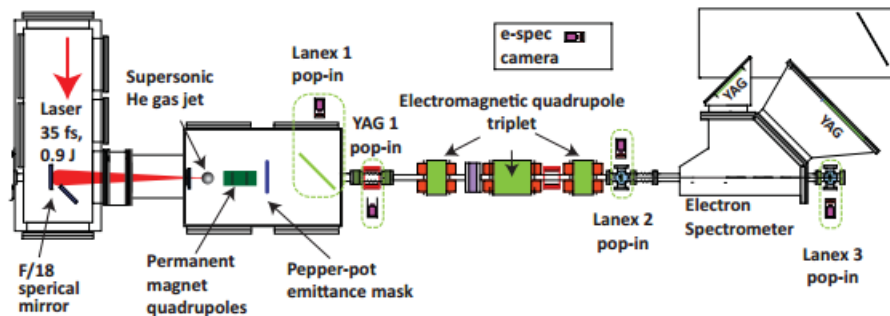
Figure 3. The ALPHA-X beamline.
