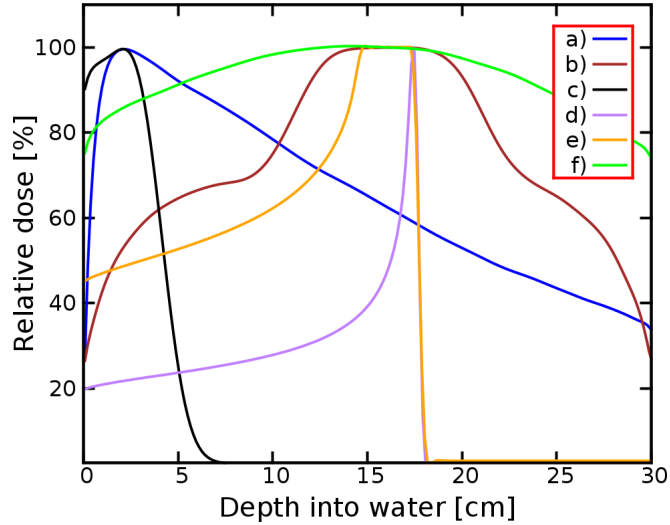
Figure 1. The percentage depth-dose distribution for different types of radiation: photons 6 MV (a), superposition of 25 MV parallel opposed photon beams and perpendicular beam (b), 10 MeV electrons (c), protons 160 MeV (d) spread-out-Bragg-peak (e), 150 MeV electrons (f).
