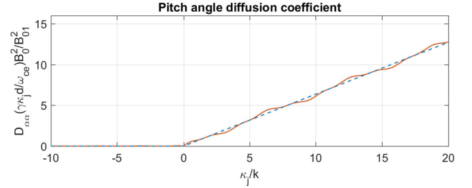
Figure 5. Normalized pitch angle diffusion coefficient
