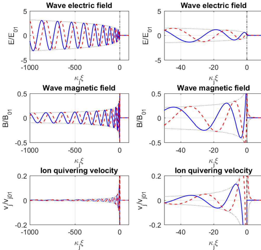
Figure 2. The electric field, magnetic field, and ion quivering velocity (top to bottom panels), showing real parts (blue solid lines) and imaginary parts (red dashed lines) near the resonance layer at \xi = 0 for a linearly decreasing magnetic field. The right-hand column shows a close-up near the resonance. The EMIC wave is evanescent and the amplitude decreases exponentially with distance for \xi > 0 .
