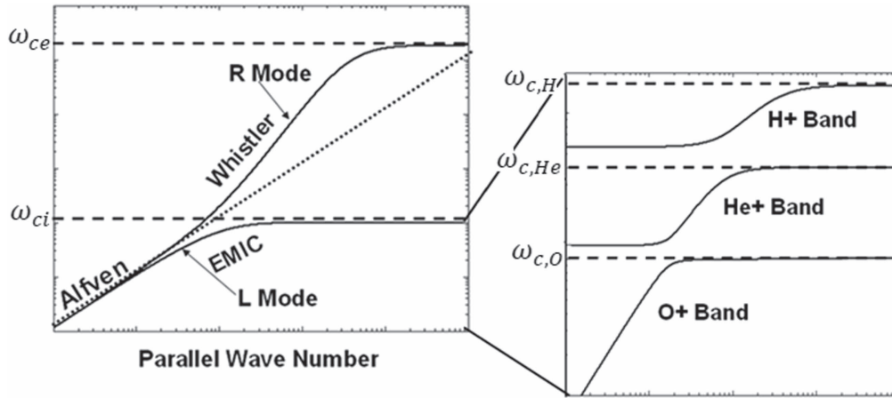
Figure 1. EMIC dispersion relation for a multi-ionic plasma including hydrogen (H), helium (He) and oxygen (O) ions.
