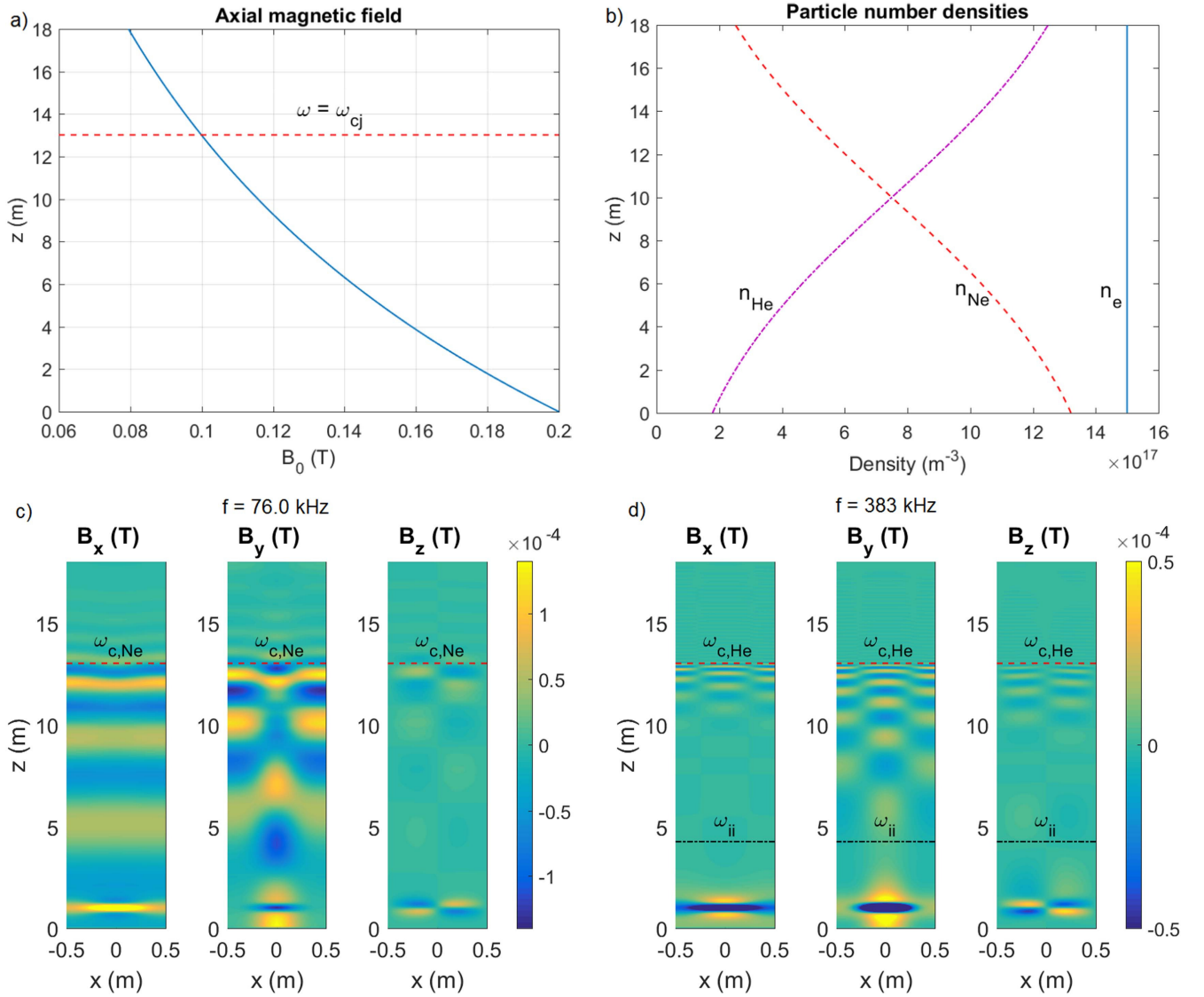
Figure 4. The propagation of EMIC waves in two-ion Ne-He plasma showing (a) the axial magnetic field, (b) particle number densities, with n_e = 1.5 \times 10^{18} \text{ m}^{-3} with spatially varying ion number densities keeping n_{\text{Ne}} + n_{\text{He}} = n_e . L-polarized EMIC waves are excited at z = 1 \text{ m} , with frequencies \omega = 4.77 \times 10^5 \text{ s}^{-1} ( f = 76 \text{ kHz} ) (panel (c)) and \omega = 4.82 \times 10^6 \text{ s}^{-1} ( f = 383 \text{ kHz} ) (panel (d)) which respectively equal \omega_{c,\text{Ne}} and \omega_{c,\text{He}} at z \approx 13 \text{ m} where B = 0.1 \text{ T} (horizontal dashed lines). The ion–ion hybrid cutoff \omega = \omega_{ii} = \sqrt{(\omega_{c,\text{Ne}}^2 \omega_{p,\text{He}}^2 + \omega_{c,\text{He}}^2 \omega_{p,\text{Ne}}^2)} / (\omega_{p,\text{Ne}}^2 + \omega_{p,\text{He}}^2) is at z \approx 4.3 \text{ m} for f = 383 \text{ kHz} (panel (d), dashed–dotted line). For clarity, the horizontal axes have been enhanced in panels (c) and (d).
