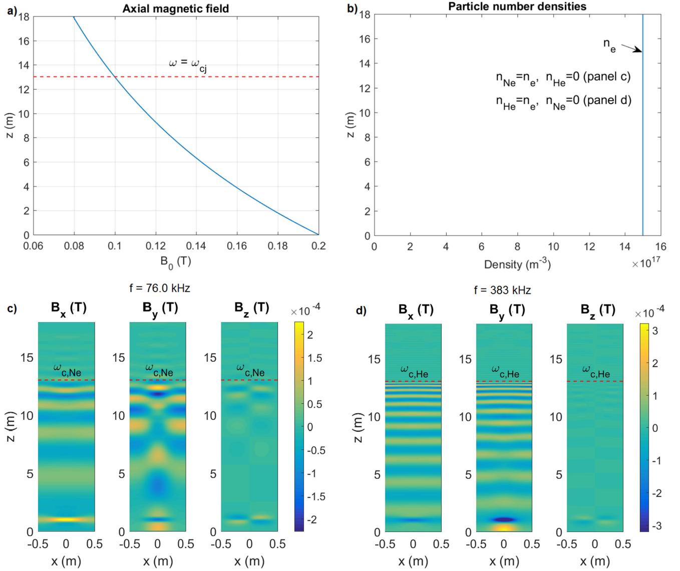
Figure 3. The propagation of EMIC waves in single ion Ne and He plasmas, showing (a) the axial magnetic field, (b) particle number densities, with n_e = 1.5 \times 10^{18} \text{ m}^{-3} and with n_{\text{Ne}} = n_e, n_{\text{He}} = 0 in panel (c) and n_{\text{He}} = n_e, n_{\text{Ne}} = 0 in panel (d). L-polarized EMIC waves are excited at z = 1 \text{ m} , with frequency \omega = 4.77 \times 10^5 \text{ s}^{-1} ( f = 76 \text{ kHz} ) (panel (c)) and \omega = 4.82 \times 10^6 \text{ s}^{-1} ( f = 383 \text{ kHz} ) (panel (d)), which respective equal \omega_{c,\text{Ne}} and \omega_{c,\text{He}} at z \approx 13 \text{ m} where B = 0.1 \text{ T} (dashed horizontal lines). For clarity, the horizontal axes have been enhanced in panels (c) and (d).
