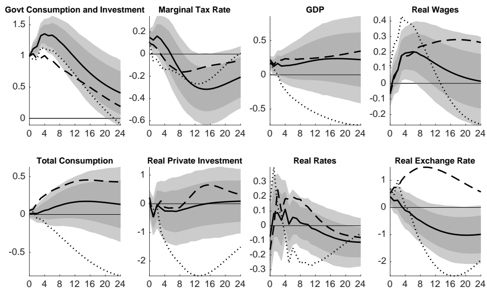
Figure 1: Fiscal Responses in Small SVAR. This figure plots the impulse response functions to a shock in aggregate government purchases (Govt Consumption and Investment) for the 1959Q1 to 2015Q4 period as solid lines with shaded posterior coverage intervals at the 0.68 and 0.9 level. Responses for subsample periods are plotted as dashed (1959Q1:1981Q4) and dotted lines (1982Q1:2015Q4) in each chart.
