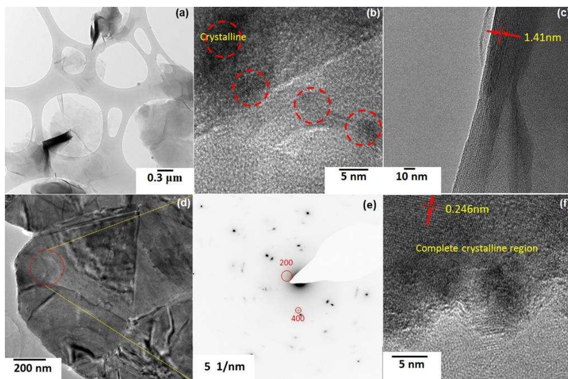
Figure 5. TEM images and electron diffraction pattern of composite adsorbents: a-c) Mont-HCF(DT0.8); d-f) Mont-HCF(DT8).
