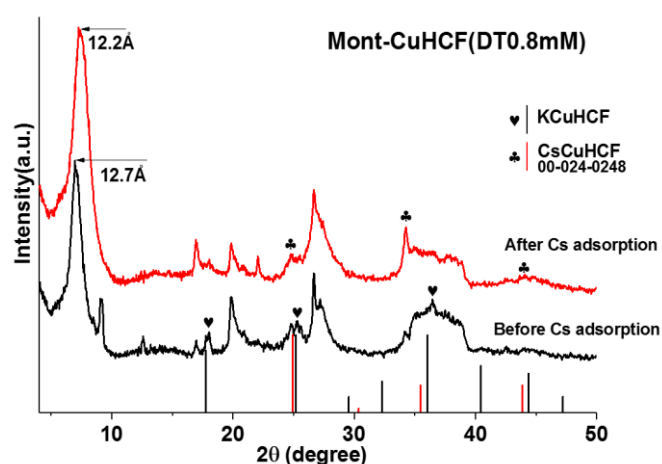
Figure 7. XRD patterns of Mont-HCF(DT0.8) before and after \text{Cs}^+ adsorption (pattern file 00-024-0248 for \text{CsCuHCF} ).
