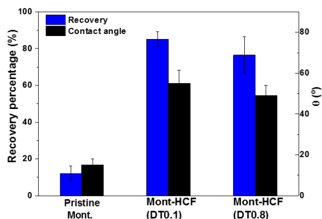
Figure 9. Flotation recovery percentages of Cs-loaded particles ( C_0 = 5 mM). The associated particle contact angles approximated by the sessile drop technique are shown on the second y-axis.
