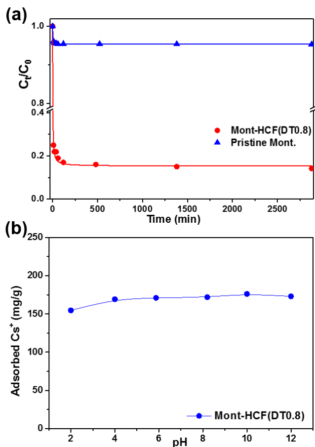
Figure 8. a) \text{Cs}^+ uptake kinetics for organo-clay-HCF composites, and pristine montmorillonite ( C_0 = 1 \text{ mM} ). b) \text{Cs}^+ adsorption as a function of the solution pH ( C_0 = 5 \text{ mM} ).
