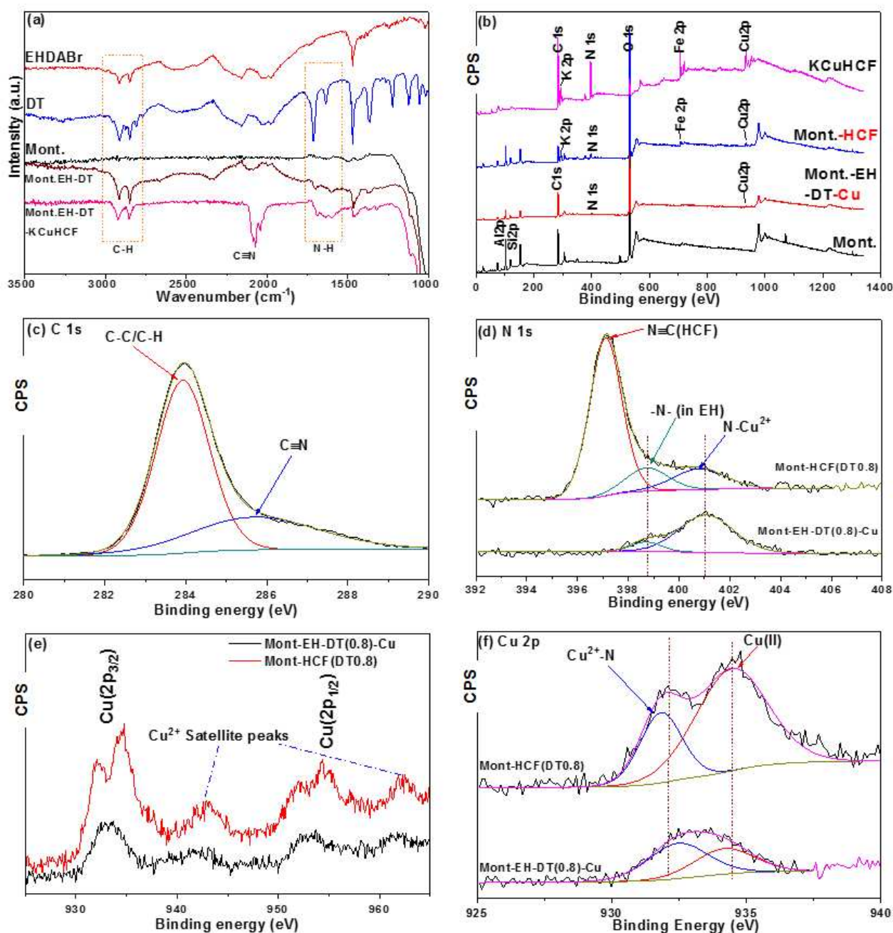
Figure 3. a) FTIR spectra of Mont-HCF composite and the intermediate product Mont-EH-DT of Step i, including the individual components Mont., EH, and DT as reference. b) XPS survey spectra (full range) of Mont-HCF composite and the intermediate product Mont-EH-DT-Cu of Step ii, with Mont. and KCuHCF shown as reference. c) High-resolution XPS spectrum on C 1s peak of Mont-HCF(DT0.8). d-f) High-resolution XPS spectra on N 1s and Cu 2p peaks of Mont-EH-(DT0.8)-Cu and Mont-HCF(DT0.8).
