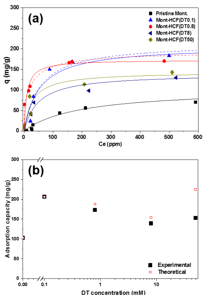
Figure 6. a) \text{Cs}^+ adsorption isotherm as a function of the equilibrium concentration ( C_e ) for Mont-HCF composites and pristine montmorillonite. Solid and dashed lines represent fittings by the Langmuir model (solid) and Dual-site Langmuir model (dashed). b) Comparison between the experimental and theoretical maximum adsorption capacities, q_m , for Mont-HCF composite particles as a function of DT concentration.
