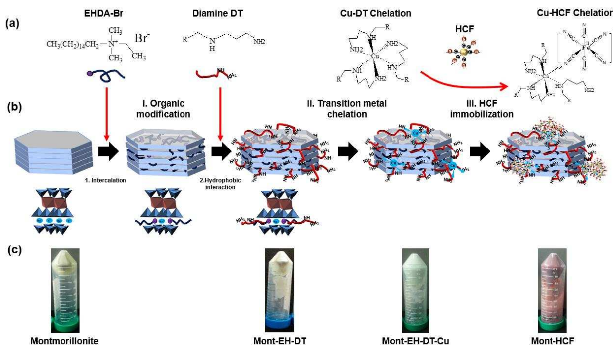
Figure 1. a) Structures of surfactant EHDA-Br, Diamine DT, along with its chelation of copper, and the association with (HCF). b) Schematic representation of the three stage preparation procedure to form-organo-clay-HCF composite adsorbent material: i) organic modification including EH intercalation and hydrophobic interaction; ii) chelation and iii) immobilization. c) Representative photos of wet samples at each stage of the preparation procedure. From left to right: Montmorillonite, Mont-EH-DT, Mont-EH-DT-Cu and Mont-EH-DT-KCuHCF (i.e. Mont-HCF).
