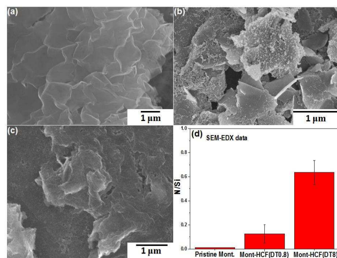
Figure 4. SEM images of a) pristine montmorillonite, b) Mont-HCF(DT0.8), c) Mont-HCF(DT8) composites, and d) N/Si ratio determined from SEM-EDX analysis.
