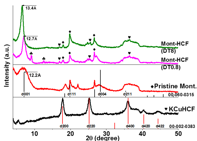
Figure 2. XRD patterns of Mont-HCF composite adsorbents with DT loadings of 0.8 mM and 8 mM. Pristine Mont. (pattern file JCPDS-ICDD 00-060-0315), and bulk KCuHCF nanoparticle (pattern file JCPDS-ICDD 02-0383) shown as reference. ♦ symbol: peaks associated with clay textural changes.
