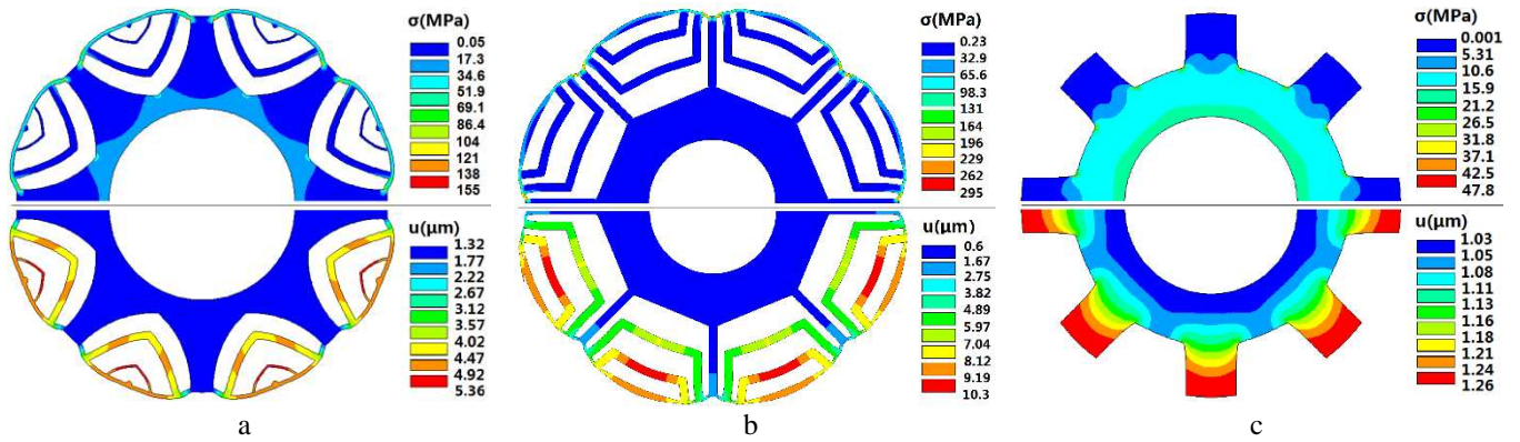
Fig. 3. Mechanical stress \sigma and radial displacement u comparison between different 8-pole rotors at 19000 rpm. a SynRM with RFBs b SynRM with AFBs c DSRM
