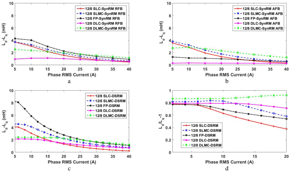
Fig. 4. Comparison of (L_d - L_q) and (\frac{L_d}{L_q} - 1) against phase RMS current between 12/8 reluctance machines. The machines
