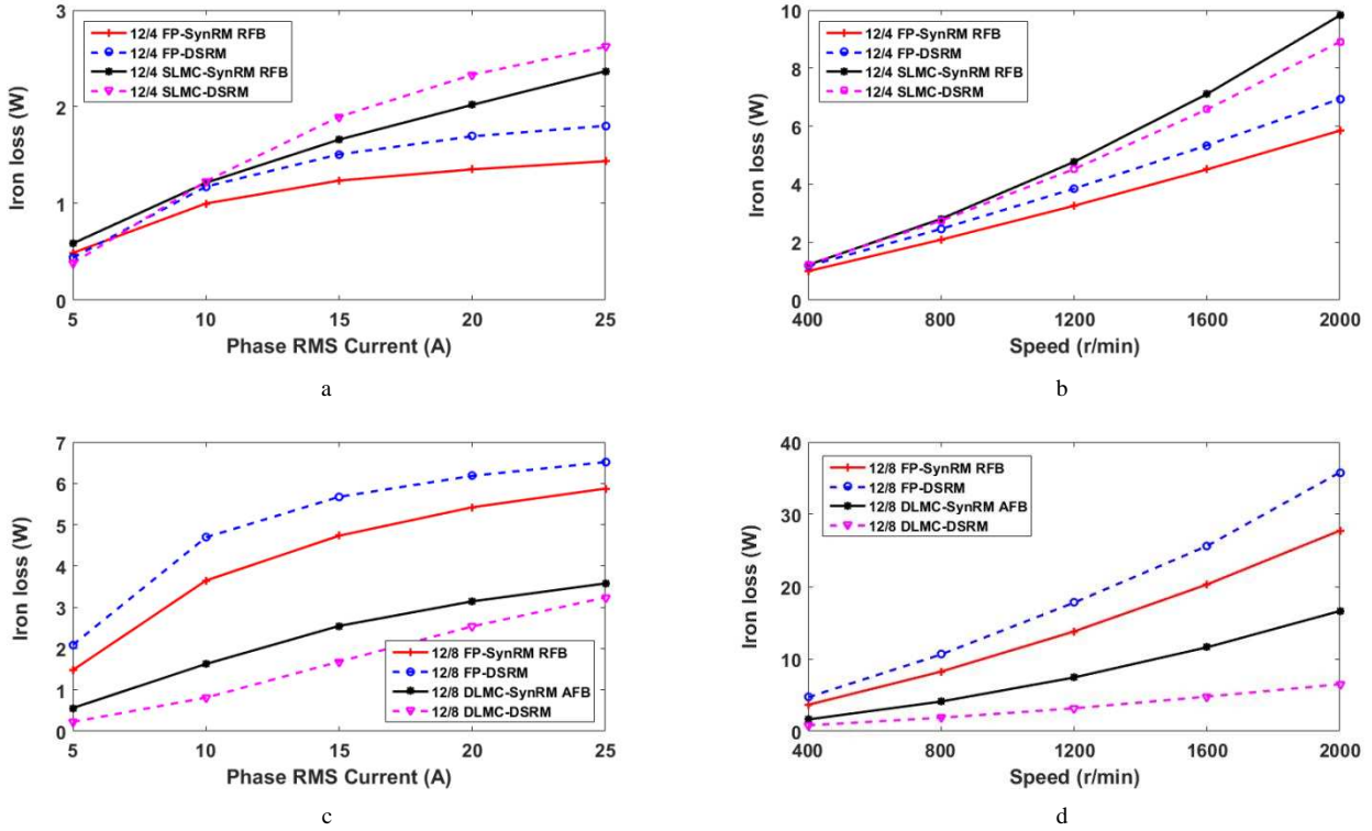
Fig. 8. Iron loss of selected 12/4 and 12/8 machines under different operating conditions. a 12/4 machines at 400 rpm with increasing phase RMS current b 12/4 machines at 10 Arms with increasing speed c 12/8 machines at 400 rpm with increasing phase RMS current d 12/8 machines at 10 Arms with increasing speed
