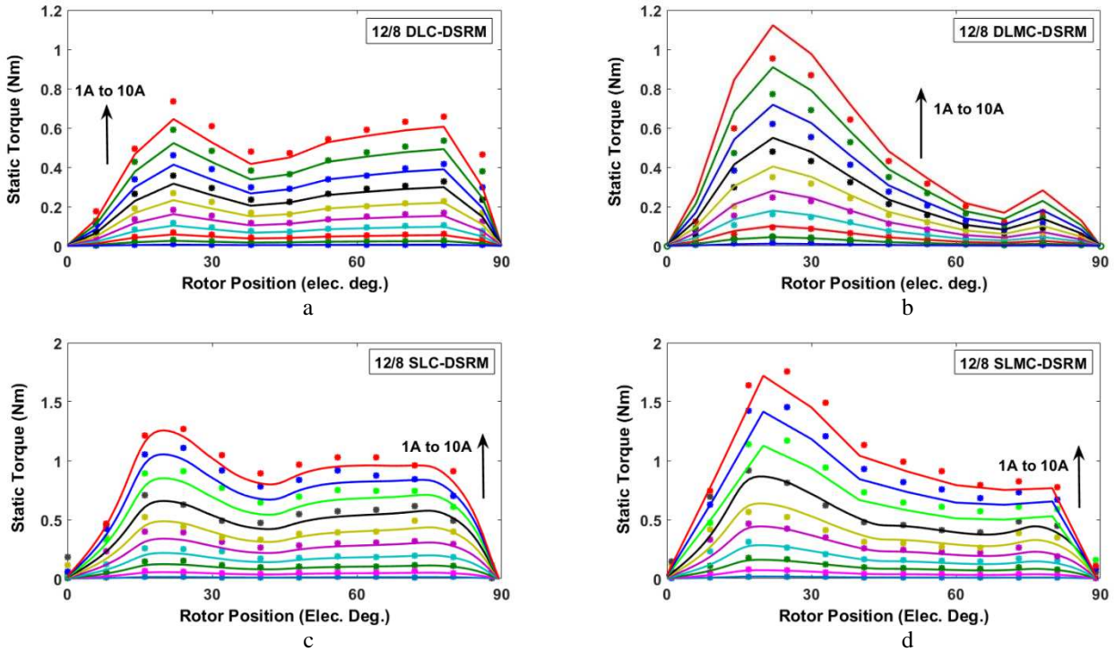
Fig. 10. Static torque against rotor position for variable currents (solid line: predicted results, dot: measured results) a 12/8 DLC-DSRM b 12/8 DLMC-DSRM c 12/8 SLC-DSRM d 12/8 SLMC-DSRM
