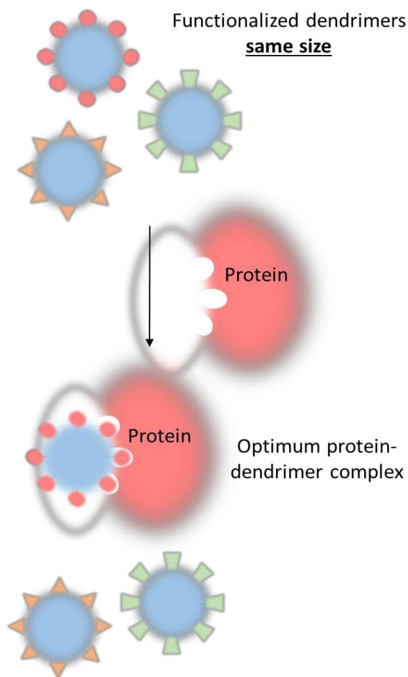
FIGURE 1 – Schematic representation showing how terminal functionality is important with respect to optimum protein binding and selectivity.
