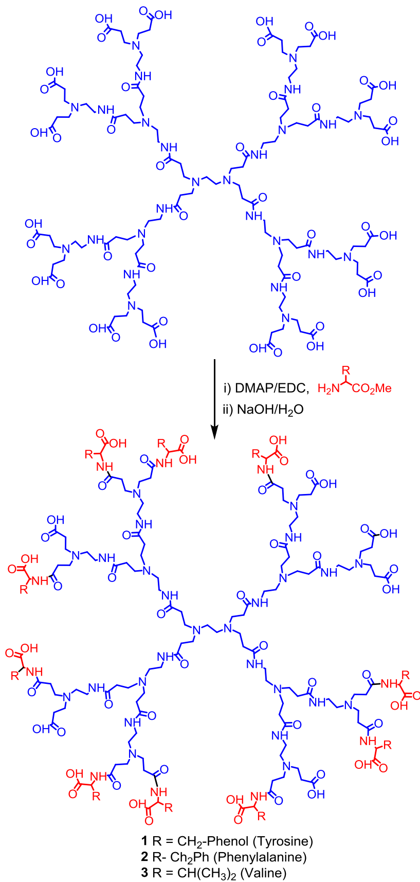
SCHEME 1: C-coupled amino acid functionalization of a G 1,5 dendrimer with 16 terminal groups.
