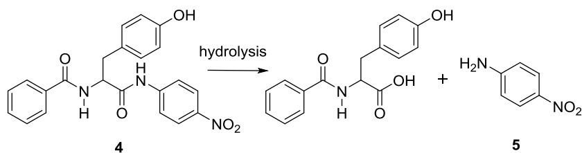
SCHEME 2: The hydrolysis reaction used to follow chymotrypsin inhibition and protein binding.
