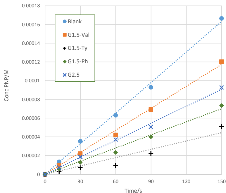
FIGURE 2: Initial rate plot for chymotrypsin/BTNA hydrolysis in the presence and absence of various dendrimers.
