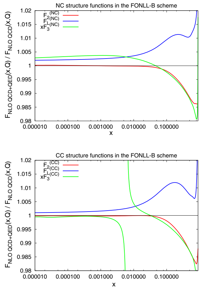
Fig. 13 The effects of the NLO QED corrections on the neutral-current (upper) and charged-current (lower plot) DIS structure functions F_2 , F_L and x F_3 , normalised to the pure QCD results. The calculation has been performed in the FONLL-B general-mass scheme using the central NNPDF3.0QED NLO set as input. Note that QED effects enter both via DGLAP evolution and the \mathcal{O}(\alpha) DIS coefficient functions. The behaviour of x F_3 in the lower plot for x \sim 0.007 is explained by the fact that this structure function exhibits a node in that region
