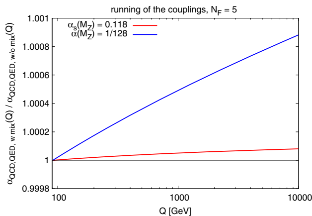
Fig. 11 Comparison between the running with the scale Q of the QCD and QED couplings, \alpha_s and \alpha , including or not the mixed terms in the corresponding \beta -functions. The curves are normalised to the result of the respective coupling running without the mixed terms included in the \beta functions
