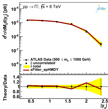
Fig. 5 Same as Fig. 3 for the highest m_{||} bin
