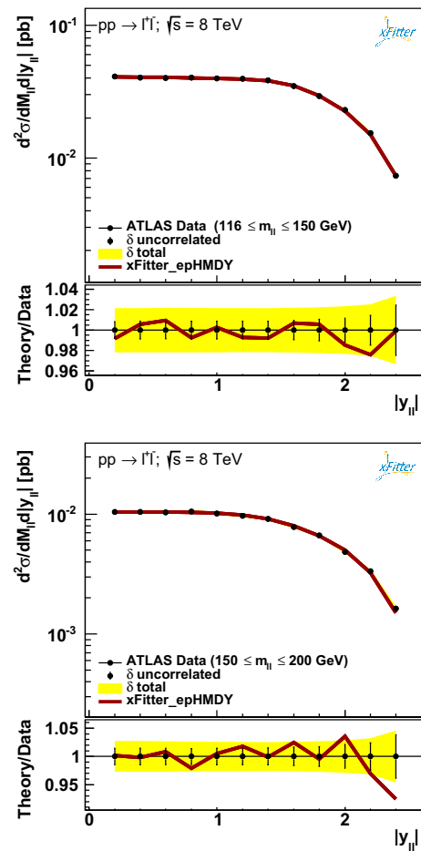
Fig. 3 Comparison between the results of the fit and the ATLAS data for the (m_{ll}, |y_{ll}|) double-differential Drell–Yan cross sections as functions of |y_{ll}| , for the first two m_{ll} bins. The comparisons are shown both in an absolute scale ( upper plots ) and as ratios to the central value of the experimental data in each y_{ll} bin ( lower plots ). The error bars on the data points correspond to the bin-to-bin uncorrelated uncertainties, while the yellow bands indicate the size of the correlated uncertainties. The solid lines indicate the theory calculations obtained using the results of the fit xFitter_epHMDY
