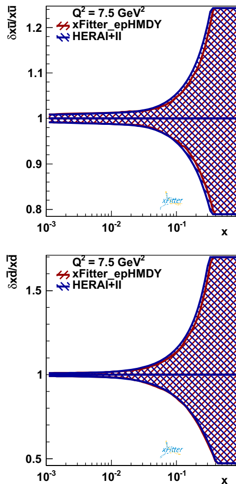
Fig. 7 The impact of the ATLAS high-mass 8 TeV Drell–Yan measurements on the x\bar{u} and x\bar{d} sea-quark PDFs at the input parametrisation scale Q^2 = 7.5 \text{ GeV}^2 . The results are shown normalised to the central value of xFitter_epHMDY .
