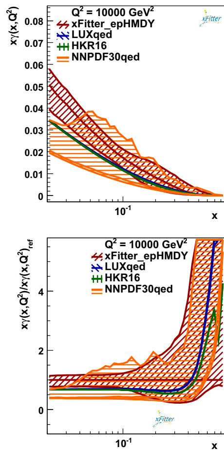
Fig. 6 Upper plot Comparison between the photon x\gamma(x, Q^2) at Q^2 = 10^4 \text{ GeV}^2 from the present NNLO analysis (xFitter_epHMDY) with the corresponding results from NNPDF3.0QED, LUXqed and HKR16. Lower plot The same comparison, now with the results normalised to the central value of xFitter_epHMDY. For the present fit, the PDF uncertainties are shown at the 68% CL obtained from the MC method, while model and parametrisation uncertainties are discussed below. For HKR16 only the central value is shown, while for LUXqed the associated PDF uncertainty band [7] is included
