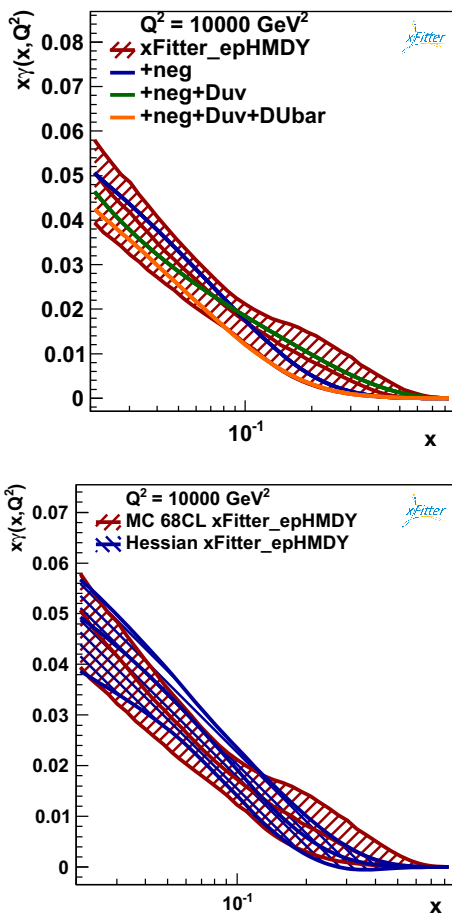
Fig. 9 Upper plot The impact on the photon PDF x\gamma(x, Q^2) from xFitter_epHMDY in fits where a number of additional free parameters are allowed in the PDF parametrisation Eq. (3). The parametrisation variations that have been explored are: more flexibility to the gluon distribution, allowing it to become negative (labeled by “neg”), adding on top D_{u_v} , and then adding D_{\bar{u}} + D_{\bar{d}} . Lower plot Comparison between the xFitter_epHMDY determinations obtained with the Monte Carlo (baseline) and with the Hessian methods, where in both cases the PDF error band shown corresponds to the 68% CL uncertainties
