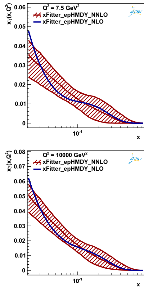
Fig. 10 Upper plot comparison between the reference xFitter_epHMDY fit of x\gamma(x, Q^2) , based on NNLO QCD and NLO QED theoretical calculations, with the central value of the corresponding fit based on NLO QCD and QED theory, at Q^2 = 7.5 \text{ GeV}^2 . In the former case, only the experimental Monte Carlo PDF uncertainties are shown. Lower plot Same comparison, now presented at the higher scale of Q^2 = 10^4 \text{ GeV}^2
