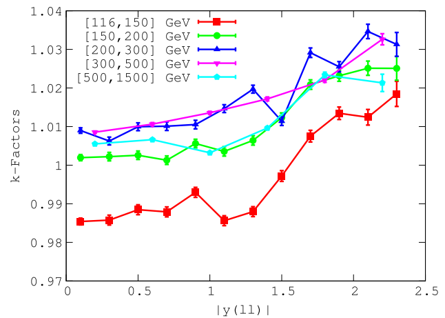
Fig. 2 The NNLO/NLO K -factors, defined in Eq. (1), which account for higher-order QCD and EW effects to the high-mass Drell–Yan cross sections with the photon-induced contribution subtracted, as a function of the dilepton rapidity |y_{ll}| . Each set of points corresponds to a different bin in the dilepton invariant mass m_{ll}
