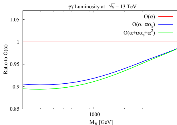
Fig. 12 The photon–photon PDF luminosity \mathcal{L}_{\gamma\gamma} at \sqrt{s} = 13 TeV as a function of the final-state invariant mass M_X . The results with the photon evolved with only the \mathcal{O}(\alpha) corrections are compared with the corresponding results taking into account the \mathcal{O}(\alpha + \alpha_s\alpha) corrections and the complete \mathcal{O}(\alpha + \alpha_s\alpha + \alpha^2) effects, normalised in all three cases to the \mathcal{O}(\alpha) result. The calculation has been performed using the central value of the NNPDF3.0QED NLO fit
