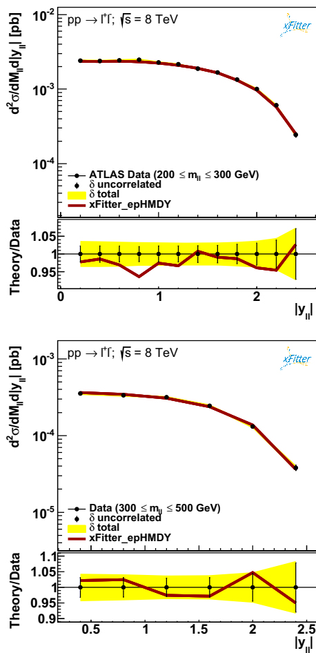
Fig. 4 Same as Fig. 3 for the third and fourth m_{||} bins
