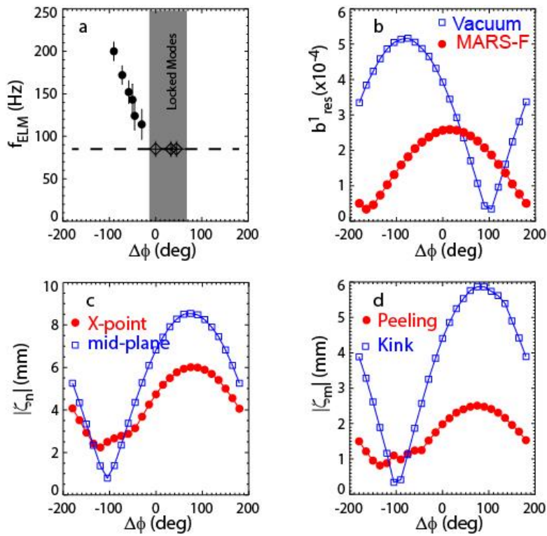
Figure 9 a) ELM frequency ( f_{\text{ELM}} ) b) normalized resonant component of the applied field ( b^1_{\text{res}} ) in the vacuum (squares) and including the plasma response (circles) c) the X-point (circles) and mid-plane (squares) displacement and d) the maximum plasma displacement normal to the flux surfaces for the kink ( m=1-4 ) (squares) and peeling ( m=6-17 ) (circles) versus the toroidal phase ( \Delta\phi ) between the upper and lower row of coils for the RMPs in an n = 3 configuration.
