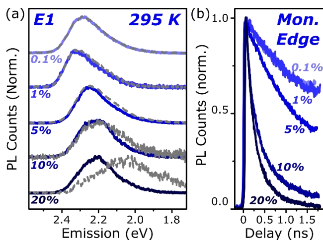
Figure 5 - Loading-dependent excimer formation. (a) Streak-camera spectra taken at 50 ps (solid) and 1500 ps (dashed) for E1 films from 0.1% to 20% dye content. The same initial state is detected at all concentrations, with a minor red-shift for 5% and above due to the inner filter effect. Slight signs of the red-shifted excimer emission can be detected at 5% loading, but only at the highest concentration does it dominate the long-time emission. (b) Corresponding normalised PL decay kinetics taken at the high-energy edge of the monomer emission. The initial singlet state is quenched progressively faster as the concentration is increased, indicating a process governed by intermolecular transfer. Full data and equivalent measurements of A1 presented in Figs. S11-12.
