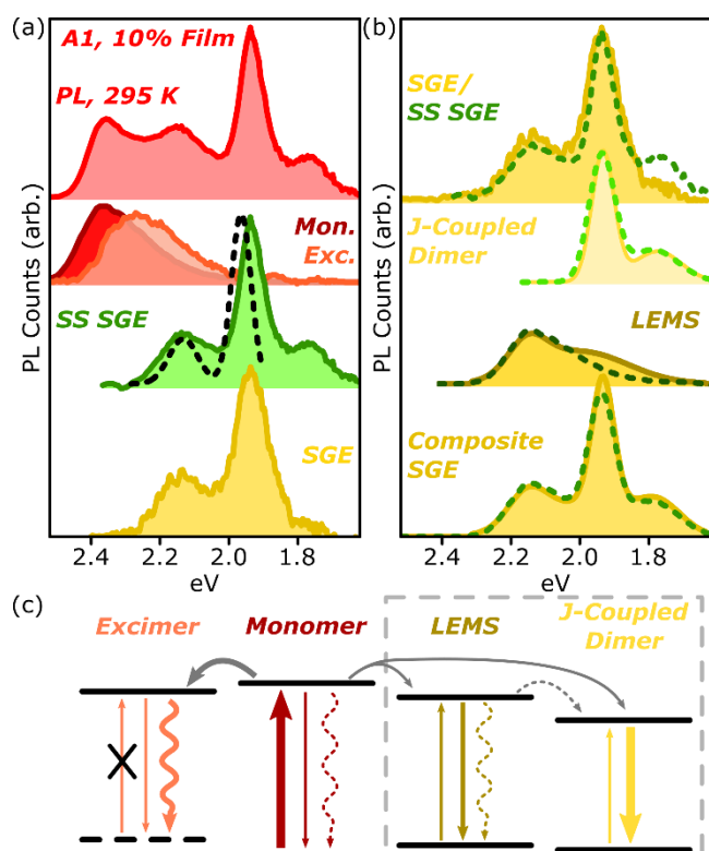
Figure 7 - Analysis of A1 spectra. (a) Room-temperature PL spectrum of 10% film (top) can be decomposed into monomer (red), excimer (orange) and steady-state (SS) sub-gap emitter (green) sub-components. The latter closely matches the SGE species identified in time-resolved measurements (yellow). PL excitation spectrum of the main SGE band (dashed) reveals that peaks at 2.15 eV and 1.95 eV must have different electronic origin. (b) Both time-resolved (filled) and steady-state (dashed) SGE spectra can be decomposed into two components. J-coupled dimer consists of two vibronic peaks with 170 meV spacing as in Fig. 2f. Residual (LEMS) closely resembles a monomer PL spectrum red-shifted by 225 meV (dashed) and broadened (filled). Reconstruction from these spectra (composite SGE) closely matches measured emission. (c) Schematic of BODIPY film photophysics. Arrows represent photon absorption or emission (straight), non-radiative decay (wavy) or energy transfer (grey). Thickness of arrows indicates relative weight of processes; dashed arrows make a weak or negligible contribution. Excimer has no defined ground state, while LEMS and J-coupled dimers can be directly photoexcited. Processes in dashed box only occur in A-type films
