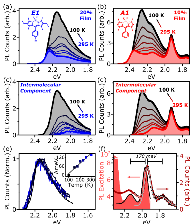
Figure 2 - Isolation of intermolecular species. Temperature-dependent PL spectra of high-concentration films of (a) E1 and (b) A1 show a strong increase in intensity upon cooling. This effect is almost entirely intermolecular, with no significant shifts or enhancement in dilute films (see ESI). Subtraction of the monomer contribution, deduced from low-concentration films and corrected for high-concentration self-absorption effects, affords the (c) E1 and (d) A1 intermolecular component, which contains the full temperature dependence. (e) The E1 intermolecular components, normalised and shifted to match peak position, exhibit the same spectral shape at every temperature. This emission arises from a single electronic species, with temperature-dependent energy and PL efficiency. Inset shows the degree each spectrum was shifted to achieve overlap. (f) PL excitation scan (filled) of the low-energy emissive peaks reveals sub-gap absorption bands with distinct vibronic structure mirrored in the PL. Sub-gap excitation at 2.14 eV (squares) and 2.0 eV (circles) yields the same low-energy emission as following excitation of the main BODIPY absorption (red line). Black and grey lines are Gaussian fits to excitation and emission spectra, giving a vibronic spacing of 170 meV.
