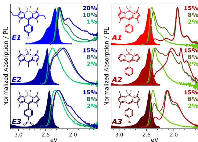
Figure 1 - Two classes of BODIPY dye. Chemical structures and normalised UV-absorption (filled) and PL spectra (lines) of BODIPY derivatives used in this study. Molecules were dispersed in polystyrene matrix, each at three different loading ratios (1 - 20% by weight in solution). In the 'E' class, increasing the concentration results in a broadening at long wavelengths, consistent with the formation of excimers. High concentrations in the 'A' class yield strongly red-shifted, highly structured spectral features consistent with ground-state aggregates. PL spectra were acquired from excitation at 473 nm.
