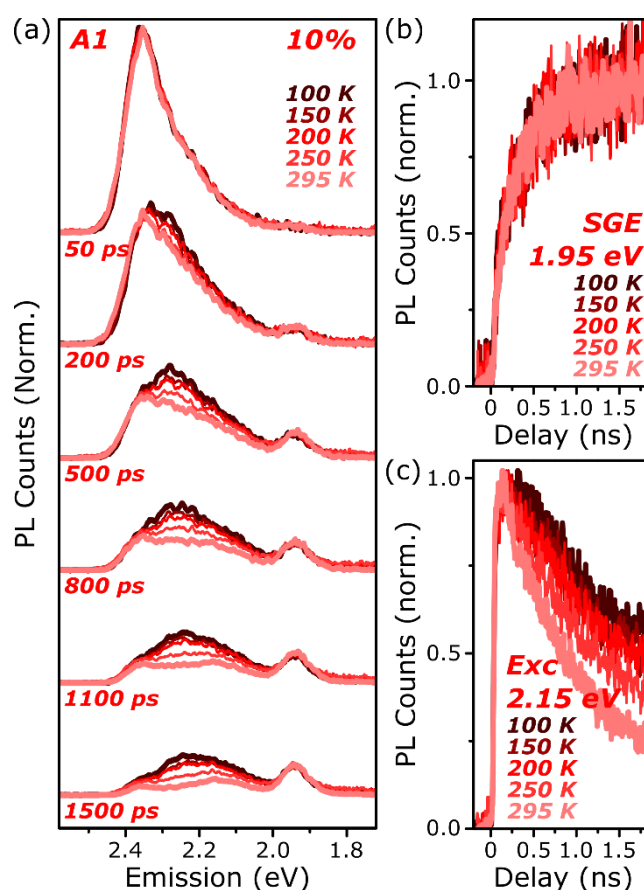
Figure 4 - Temperature-dependent excimer and aggregate dynamics. (a) Streak-camera spectra taken at the indicated delay times following photoexcitation, for an A1 film at 10% dye content held at 100-295 K. The datasets were normalised to the intensity of the initial spectral slice; no further scaling was applied for longer time delays. The yield and shape of the SGE band at 1.95 eV and shape of the monomer edge at 2.4 eV are invariant across the temperature series. Only in the intermediate excimer region is a strong dependence observed. (b) Integrated PL kinetics centered on the peak of the SGE band reveal, within measurement limits, identical dynamics at all temperatures. (c) Integrated PL kinetics from the excimer region at 2.15 eV reveal progressive enhancement of the lifetime upon cooling, consistent with a reduction in non-radiative decay rates. Full data and equivalent measurements of E1 presented in Figs. S14-15.
