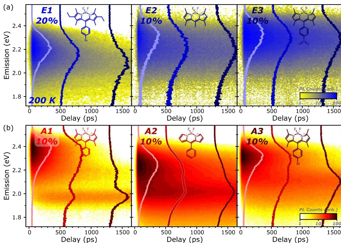
Figure 3 - Fast PL dynamics. (a) Streak-camera measurements of high-concentration E-class films, taken at 200 K (E1) or 295 K (E2, E3). Normalised spectral cuts (lines; light blue: 50 ps, blue: 200 ps, dark blue: 1500 ps) highlight the evolution of emissive species. The initial spectrum in all cases corresponds to monomer emission detected in dilute films. The final spectrum in E1 matches the excimer component identified above, and equivalent red-shifts and broadening are observed in E2 and E3. (b) Streak-camera measurements of high-concentration A-class films at 295 K. Normalised spectral cuts (lines; pink: 50 ps, red: 200 ps, dark red: 1500 ps) highlight the evolution of emissive species. Initial spectra in all films can be assigned to monomer emission similar to dilute films. The final spectrum in A1 corresponds to the temperature-independent portion of the intermolecular spectrum identified above. The spectral shape at intermediate times indicates the presence of a third, distinct species emitting in the range of the excimer identified from steady-state measurements. Comparable multi-species evolution is evident in A2 and A3. Spectral maps are presented with logarithmic intensity scale to highlight the contribution of weak, long-lived features.
