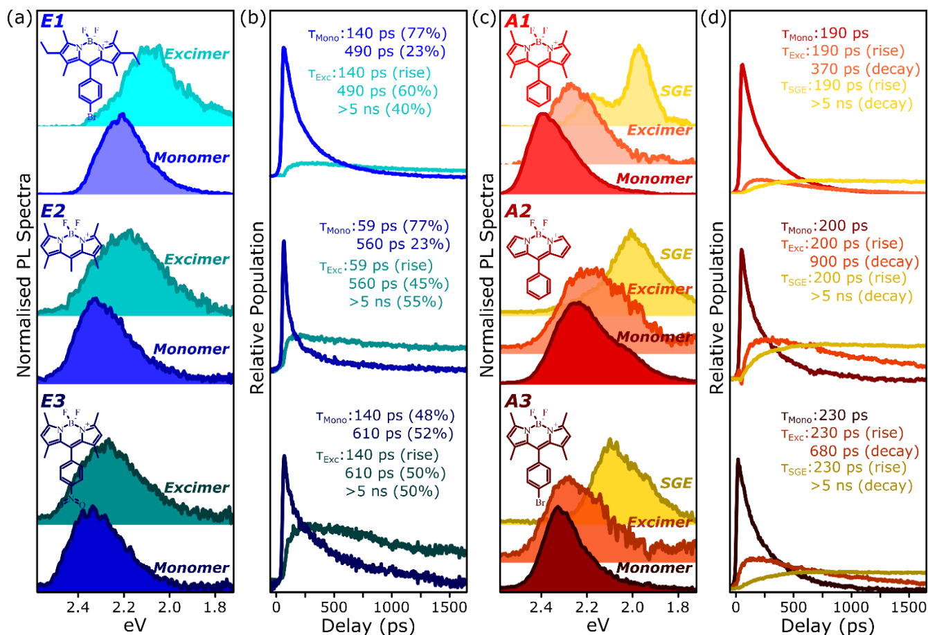
Figure 6 - PL spectral decomposition. (a) Decomposition of time-resolved PL maps of high-concentration E-class BODIPY films affords a good match with two distinct species: the initially photo-generated monomer and weakly red-shifted, structureless excimer emission. E1 data was taken from a 20% film at 200 K, E2 and E3 from 10% films at 295 K. (b) The corresponding population kinetics reveal fast monomer decay (blues) and delayed excimer formation (greens) over 10's-100's of ps, consistent with energy migration through the film. Time constants result from global multiexponential fitting. (c) Decomposition of the PL maps of high-concentration (10%) A-class BODIPY films at 295 K requires three distinct species for an adequate fit: the photo-generated monomer (reds), weakly red-shifted excimer (oranges) emission similar to that of the E class and strongly red-shifted SGE (yellows) with vibronic structure. (d) Relative population kinetics of monomer (reds), excimer (oranges) and SGE (yellow) show parallel population of long-lived SGE and shorter-lived excimer emission sites from the rapidly quenched monomer, over 10's-100's of ps. Traces reflect relative spectral intensity. Time constants result from global multiexponential fitting. The time constant of excimer growth is similar to SGE, but the fast subsequent decay results in a markedly earlier population peak.
