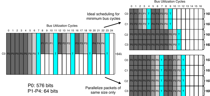
Fig. 4: Scheduling Multiple Packet Sizes
