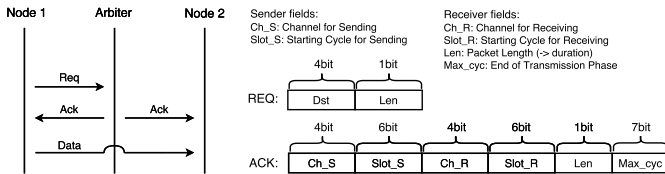
Fig. 6: Control message exchange in centralized arbitration and all possible REQ/ACK fields
