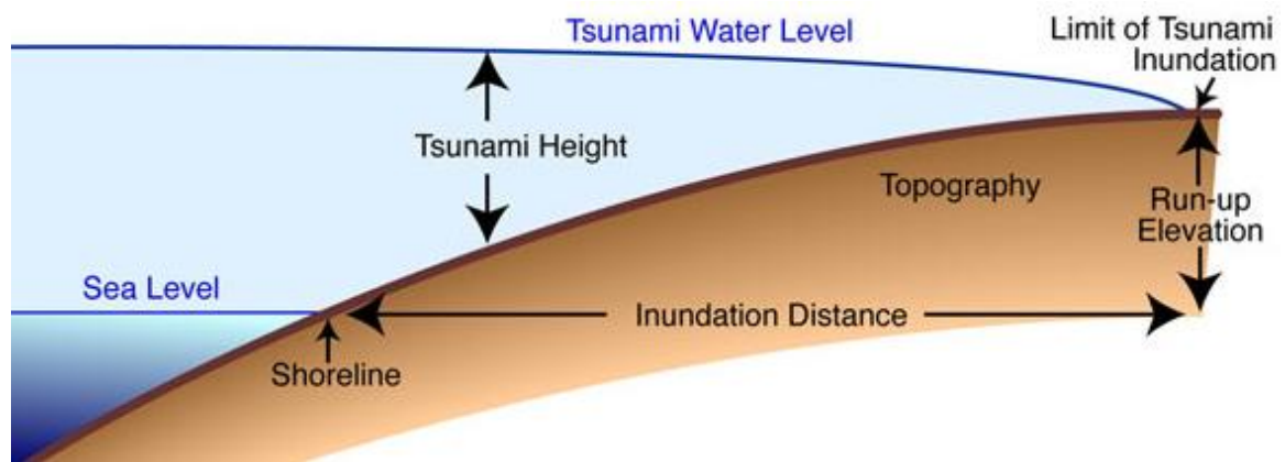
Figure 13: Tsunami Inundation Diagram Source: Discover Tsunamis 29
