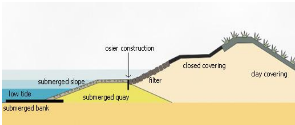
Figure 48: Sea Dike Cross Section Source: SeaOnScreen 63
