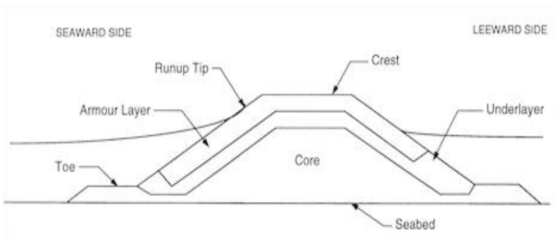
Figure 49: Cross section of sloping front breakwater Source: University of Wisconsin Madison 66
