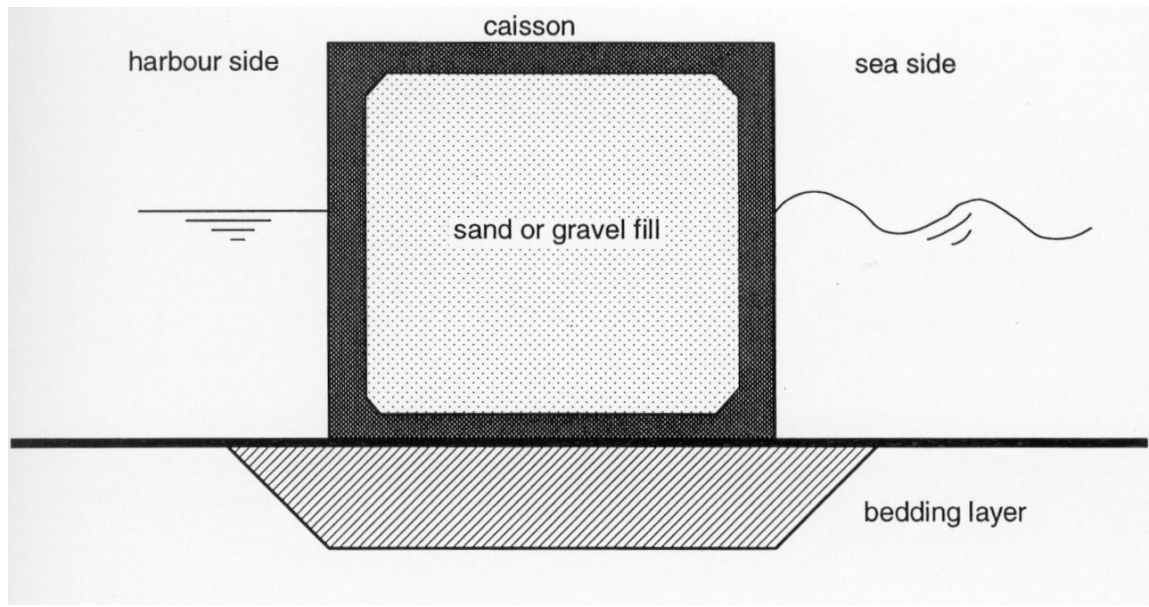
Figure 50: Cross section of vertical front breakwater Source: Kennisbank 67
