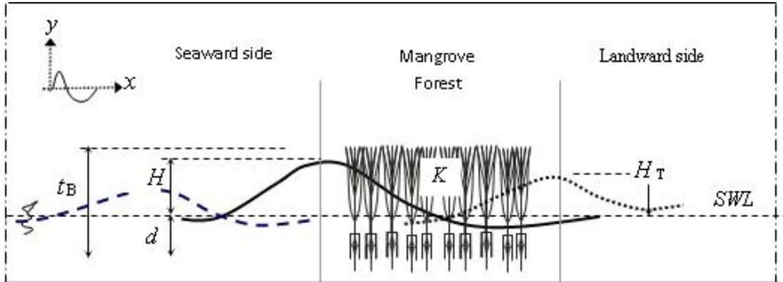
Figure 55: Mangrove Forest Sea Belt. Source: Disaster Reduction Hyperbase 77
