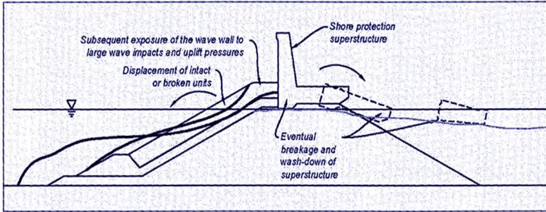
Figure 53: Diagram of Scour Mechanisms Source: American Society of Civil Engineers 74
