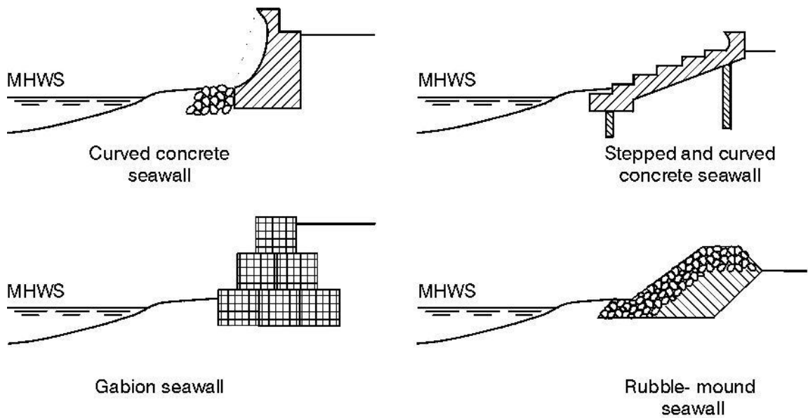
Figure 47: Examples of seawall structures Source: Coastalwiki 60
