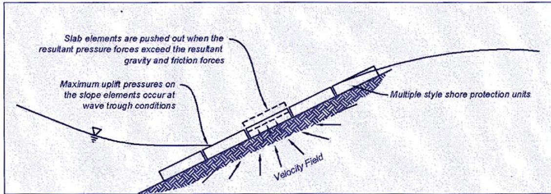
Figure 52: Hydrostatic Uplift Forces Source: American Society of Civil Engineers 72
