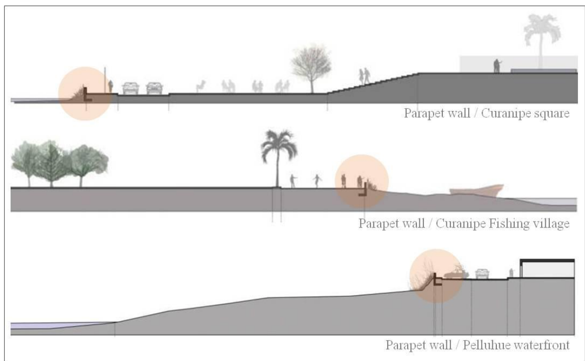
Figure 75: PRES Parapet walls interventions in Pelluhue Source: Source: PRES Pelluhue 2010 128
