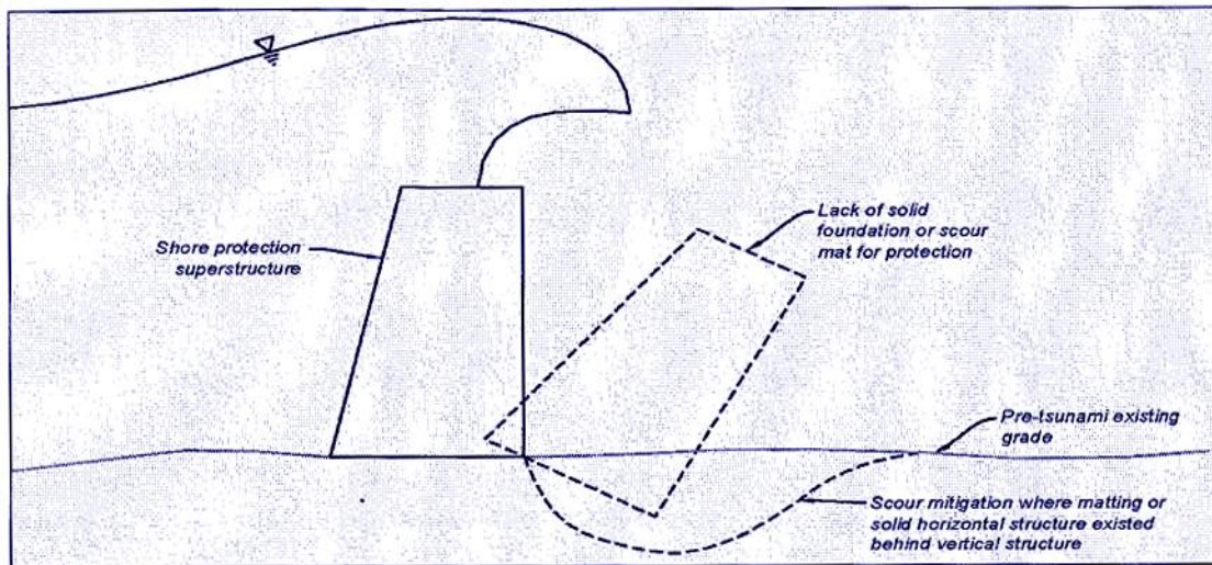
Figure 54: Erosion Diagram Source: American Society of Civil Engineers 75
