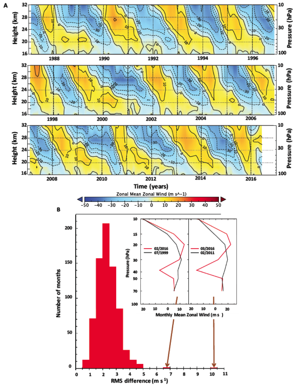
Fig. 1. Evolution of the QBO showing regular repeating wind structures and anomalous westward winds in 2016. (A) Vertical profile time series of monthly mean zonal mean eastward wind averaged over 5°S-5°N showing descending eastward (yellow) and westward (blue) wind regimes (24) for the last thirteen observed QBO cycles. (B) Histogram of root mean square (rms) differences in monthly-mean eastward wind averaged over the 70, 50, 40, 30, 20, 15 and 10 hPa levels between each of the 724 monthly profiles from all 27 observed QBO cycles and its closest match in the record (11). Only matches between profiles separated by more than six months were evaluated to ensure only matches from earlier or later QBO cycles were considered. The inset panels show monthly-mean profiles together with their best matches for February and March 2016.
