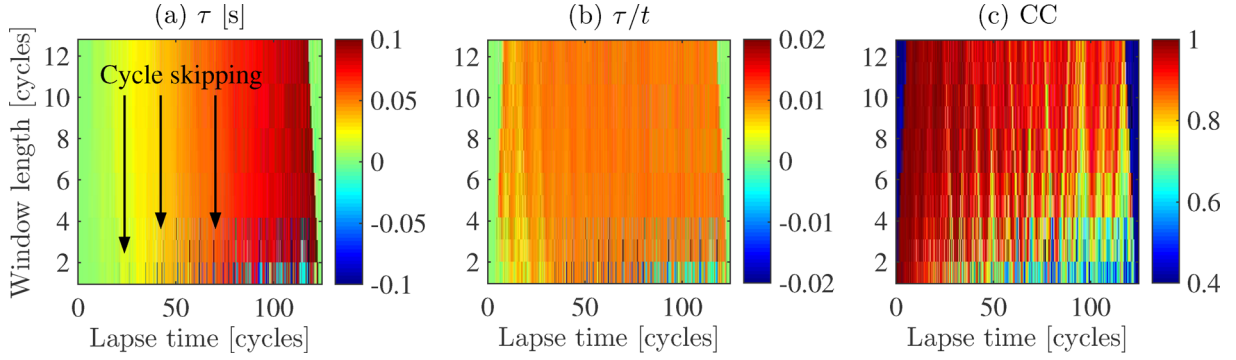
Figure 4. (a) The lag \tau at each lapse time for the varying window lengths in the sliding window cross-correlation method. (b) The time normalized lag giving an estimate of homogeneous negative velocity perturbation. (c) The maximum correlation coefficient for each window length.
