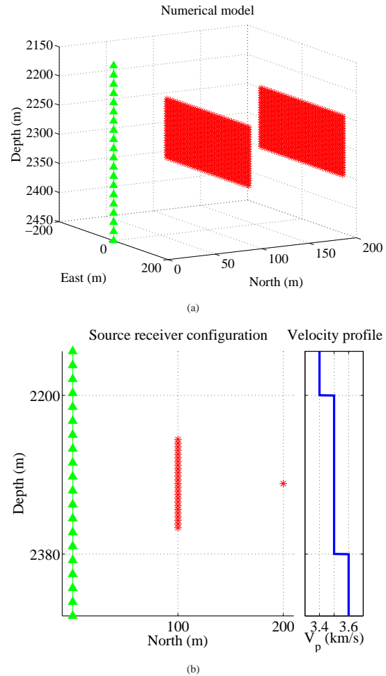
Figure 5: The numerical model contains a monitoring well with two vertical fractures nearby. A source in the more distant fracture is localized using 625 microseismic sources in the nearer fracture.
