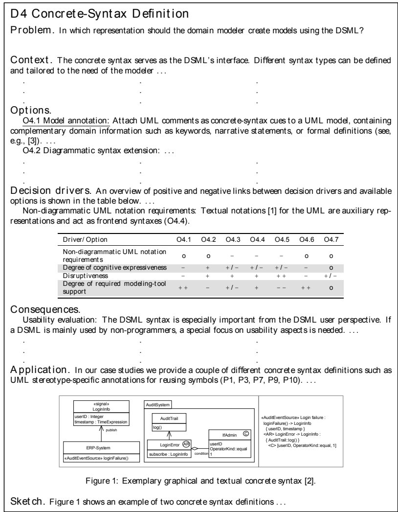
Figure 2: Excerpt from the actual decision record on concrete-syntax definition (D4) in Hoisl et al. [33], highlighting the document sections corresponding to the key concepts in Figure 3.
