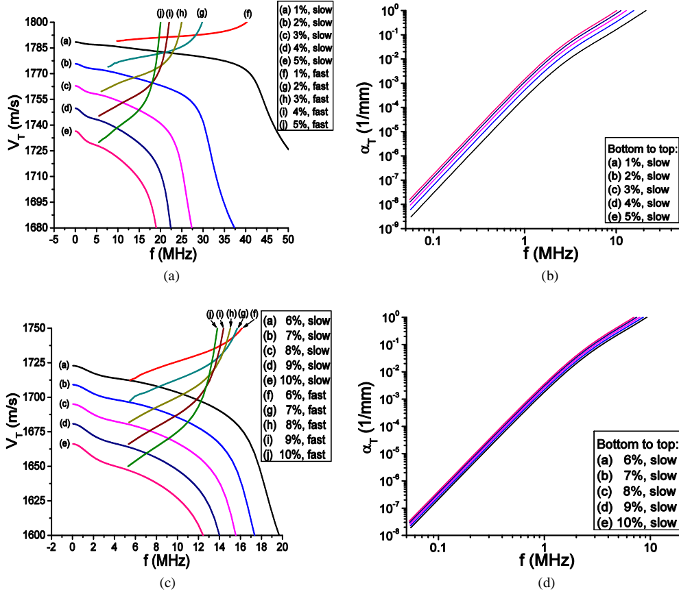
FIG. 39. Transverse dispersion (a), (c) and attenuation (b), (d) of cortical bone with different porosities: d=100 \mu\text{m} .
