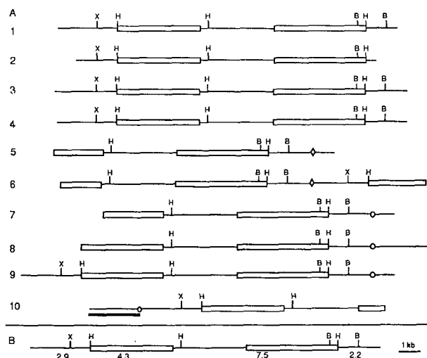
Figure 3. Restriction Maps of \lambda Clones Containing T-DNA Sequences.
