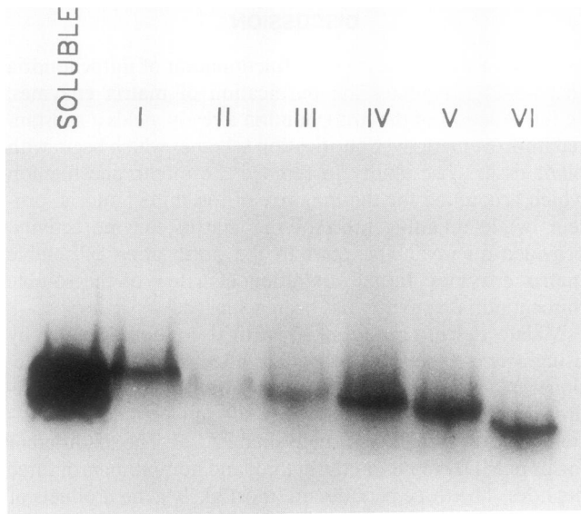
Figure 7. Separation of native MDH isoenzymes by nondenaturing PAGE. Purified MDH isoenzymes were run on 7.5% acrylamide nondenaturing gels and the gels were stained for MDH activity. The most active fraction for each isozyme from the Phenyl Superose column was concentrated and loaded.
