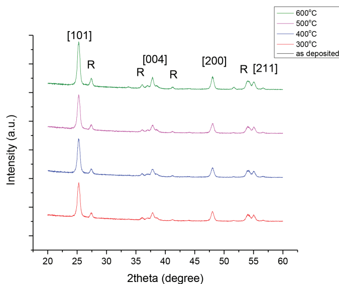
FIGURE 2. XRD spectrum of \text{TiO}_2 thin films annealed at different temperatures
