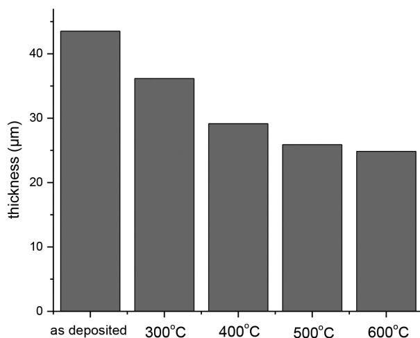
FIGURE 3. Thickness of TiO 2 thin film annealed at different temperature
