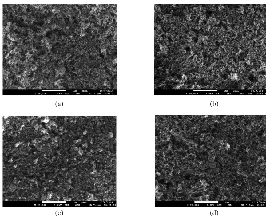
FIGURE 1. FESEM images of \text{TiO}_2 thin films annealed at (a) 300°C, (b) 400°C, (c) 500°C and (d) 600°C
