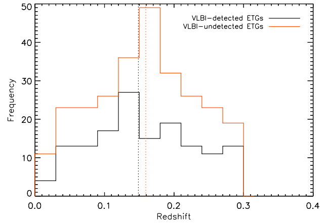
Figure 3. Left: mJIVE luminosities of VLBI detections (black) and upper limits in the VLBI non-detections (orange). Right: the redshift distribution of the VLBI detections (black) and their undetected counterparts (orange). Vertical dotted lines indicate median values.
