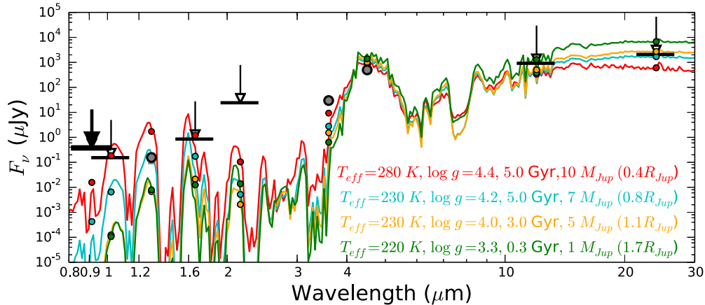
Figure 3. Burrows et al. (2003) atmospheric models for various effective temperatures T_{\text{eff}} , surface gravities \log g , and ages. Large gray filled circles are detections using WISE (Wright et al. 2010) and Spitzer , and the 2.6\sigma J -band detection by Faherty et al. (2014). Large arrows are upper brightness limits from Luhman (2014), Wright et al. (2014), and Beamín et al. (2014). The small color-coded dots are fluxes in photometric bands predicted by the models. Our upper limit is highlighted at the far left. All photometric measurements are on the AB system. The hottest model shown is ruled out both by the upper limits and by the physically implausible radius required to match the detections.
