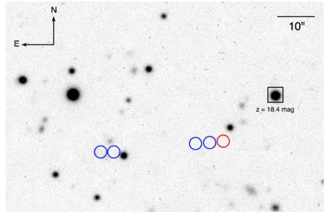
Figure 1. z -band FORS2 observations of the field containing WISE0855-07. Blue circles are WISE positions in 2010.34 and 2010.86 (the pair on the left) and Spitzer positions 2013.47 and 2014.05 (the pair on the right). The red circle is the expected position of WISE 0855-07 on 2014 May 31. No counterpart to WISE 0855-07 is detected in our z -band FORS2 frames. For reference, the square indicates a source with z(\text{AB}) = 18.4 mag.
