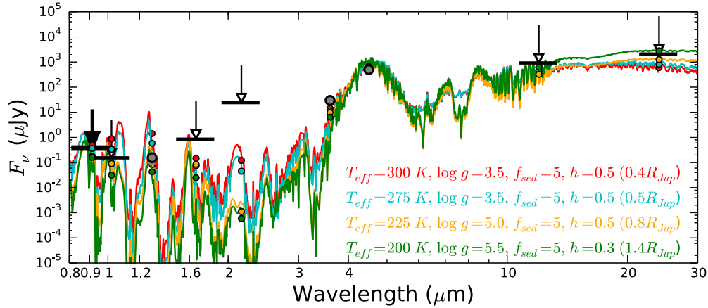
Figure 2. Morley et al. (2014) atmospheric models for various effective temperatures T_{\text{eff}} , surface gravities \log g , and cloud sedimentation parameters f_{\text{sed}} . Large gray filled circles are detections using WISE (Wright et al. 2010) and Spitzer , and the 2.6\sigma J -band detection by Faherty et al. (2014). Large arrows are upper brightness limits from Luhman (2014), Wright et al. (2014), and Beamín et al. (2014). The small color-coded dots are fluxes in photometric bands predicted by the models. Our upper limit is highlighted at far left. All photometric measurements are on the AB system. The hottest model shown is ruled out both by the upper limits and by the physically implausible radius required to match the detections.
