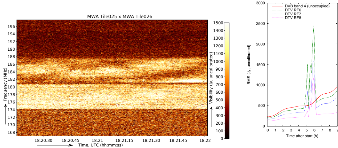
Figure 4.: RFI from digital TV (DTV), which is visible in 1 of the 9 observations (GLEAM 2014-03-17) that cover the DTV frequencies. Left plot: dynamic spectrum for the worst affected snapshot; right plot: visibility RMS in a few of the DTV bands for the affected night after flagging. Because of its broadband nature, this kind of RFI is not well-flagged in the initial AOFLAGGER step, but it is detectable in the global statistics.
