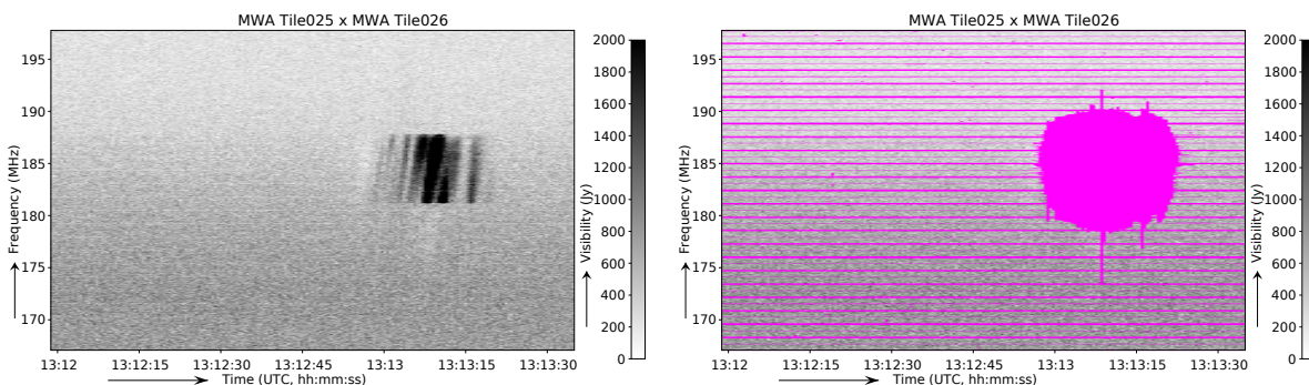
Figure 7.: DTV RFI briefly visible in an EoR high-band observation. The plots show the Stokes I amplitudes for a single correlation. The right plot shows the result of RFI detection and invalid channels marked in purple.
