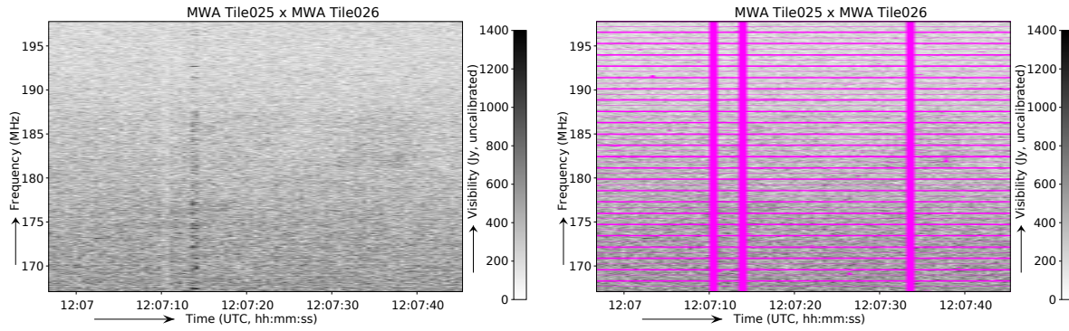
Figure 8.: Broadband pulses found in an EoR high-band observation. The two panels show Stokes I visibility amplitudes of a single correlation. In the right plot, the RFI detection flags and invalid channels are marked with purple. Each event occupies 2 timesteps of 0.5 s.
