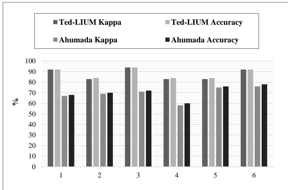
FIGURE 4.2: ACCURACY AND KAPPA MEASURES ACHIEVED BY OUR SYSTEM OVER THE 6 DATA SETS OF BOTH TED-LIUM AND AHUMADA CORPUSES
