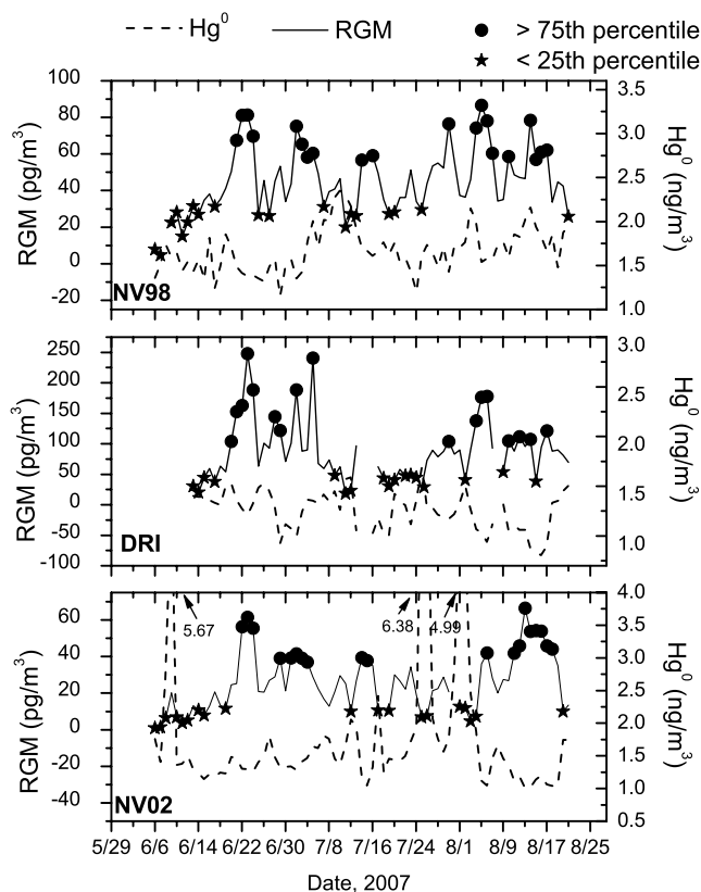
Figure 3. Time series plots of daily mean RGM and Hg 0 concentrations from NV98, DRI, and NV02. Days when RGM concentrations were <25th or >75th percentile of the daily mean distribution are highlighted with symbols. The NV02 Hg 0 plot shows peak daily mean concentrations for the three events that are off-scale.
