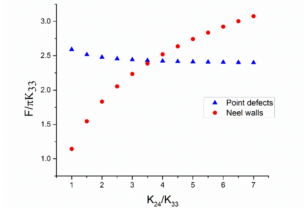
Figure 2.6 Free energy contribution of the configuration with neel walls and point defects
