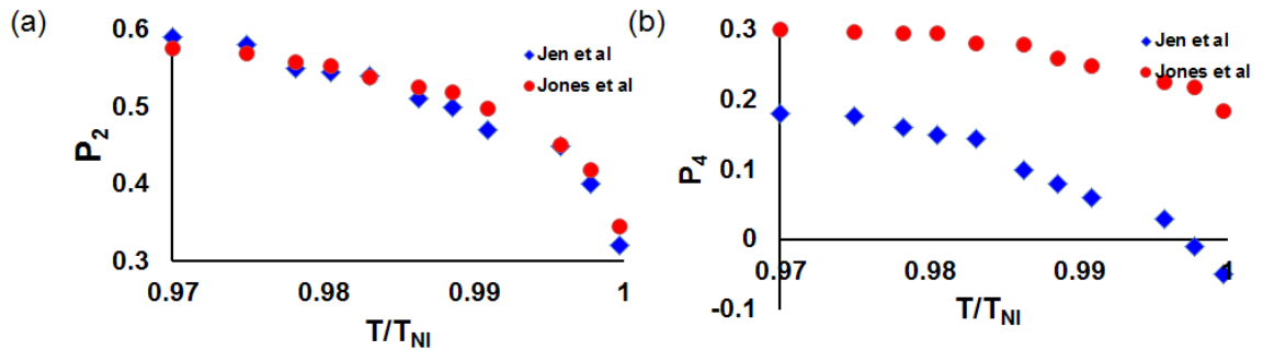
Figure 7.1 Order parameters P_2 and P_4 measured by the method of Jones et al and Jen et al
