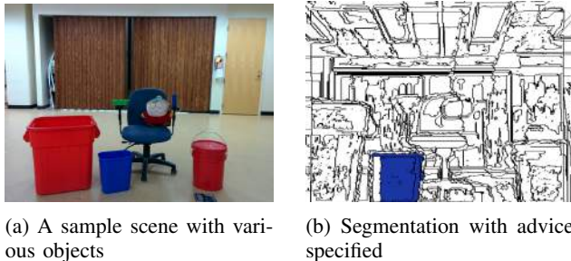
Fig. 3: Segmentation-based advice-giving
