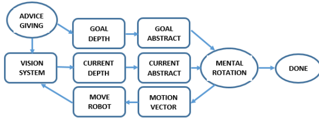
Fig. 1: Navigational algorithm architecture
