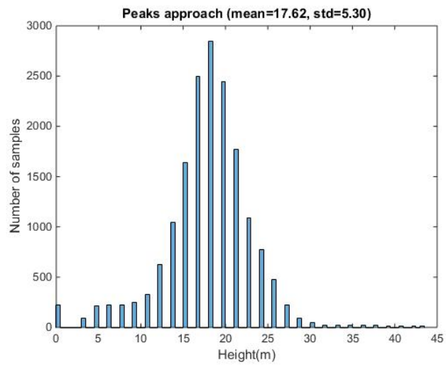
Figure 4.14: Estimated tree height histograms.
