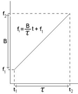
Figure 2.1: Linear chirp. Time is the x-axis and frequency the y-axis. The chirp presents a linear relationship between time and frequency.
